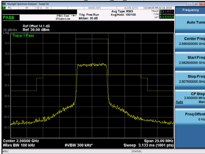
Band 38_16QAM_5M_RB1,0
