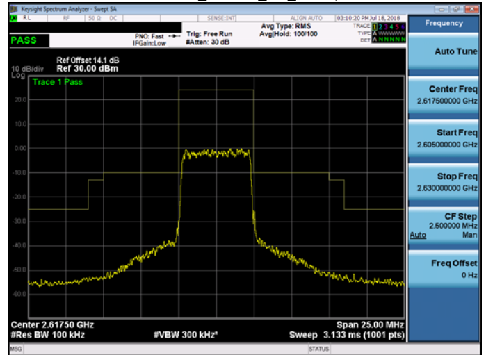
Band 38_QPSK_10M_RB1,0
