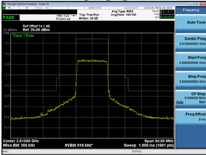
Band 38_16QAM_10M_RB1,0
