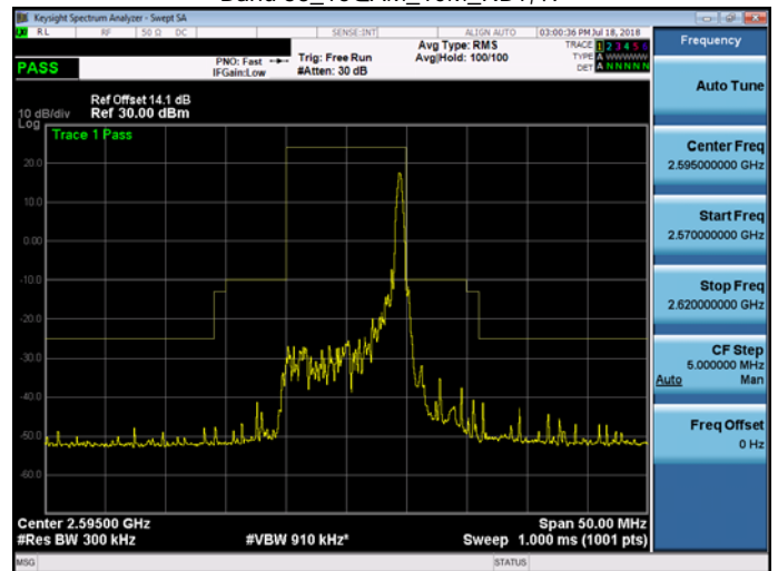
Band 38_16QAM_10M_RB1,49
