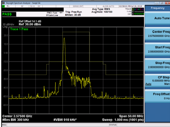
Band 38_16QAM_10M_RB1,49
