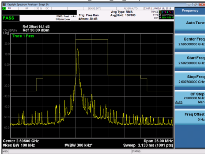
Band 38_QPSK_5M_RB1,24
