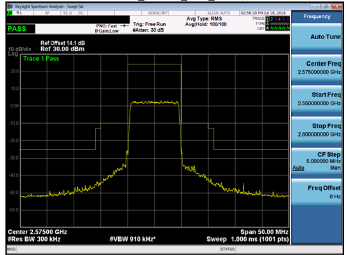
Band 38_16QAM_10M_RB1,0
