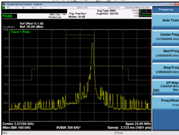
Band 38_16QAM_5M_RB1,24
