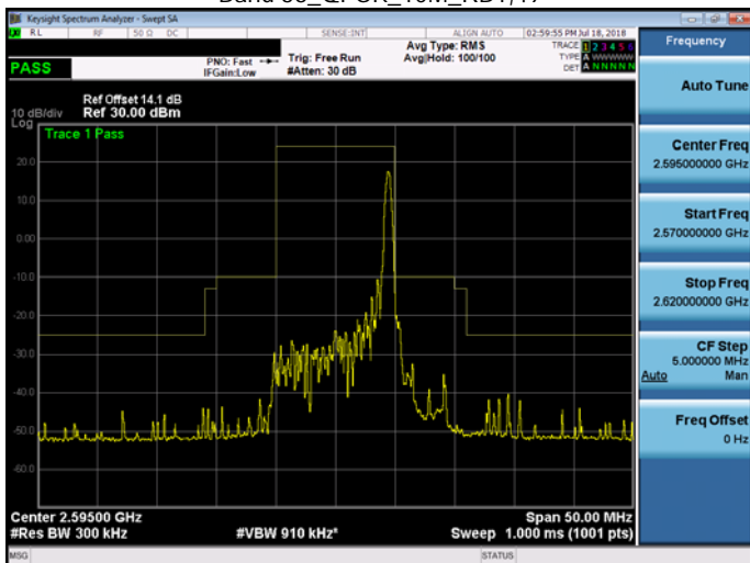
Band 38_QPSK_10M_RB1,49
