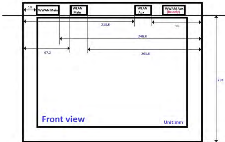
Fig.10 Antenna location of EUT (tablet mode)
