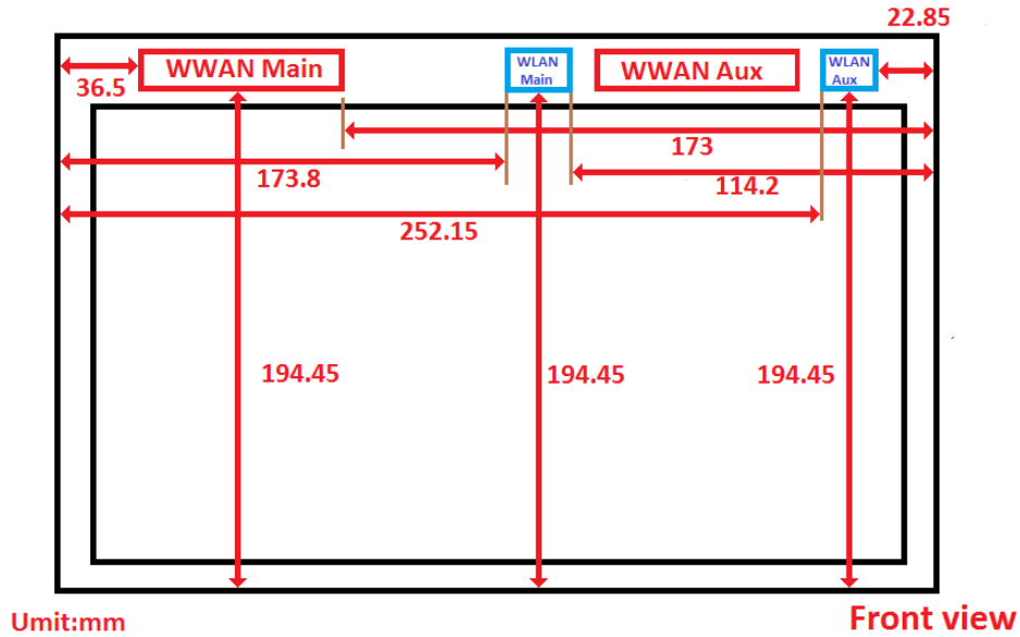
Fig.12 Antenna position of EUT
