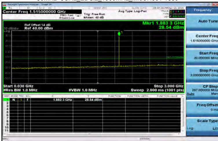
30MHz~3GHz_EDGE_1900MHz_MidCH661-1880
