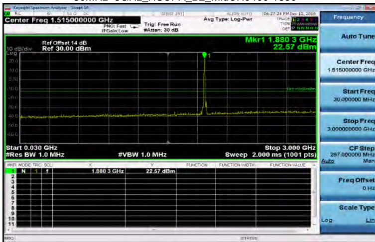
30MHz~3GHz_HSUPA_B2_MidCH9400-1880
