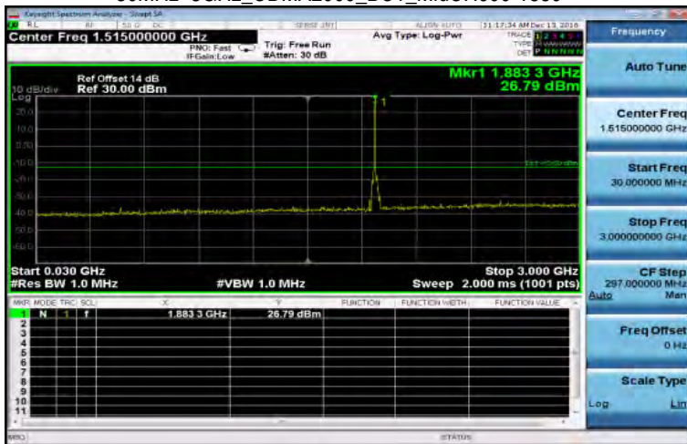
30MHz~3GHz_CDMA2000_BC1_MidCH600-1880
