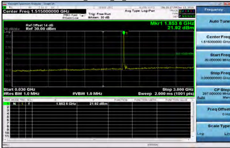
30MHz~3GHz_HSUPA_B2_LowCH9262-1852.4
