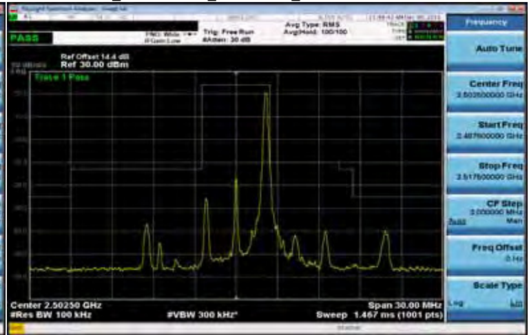
Mask_Band7 5MHz_QPSK 1 24_LowCH20775-2502.5
