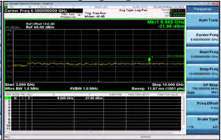
3GHz-10GHz_GPRS_850MHz_MidCH190-836.6
