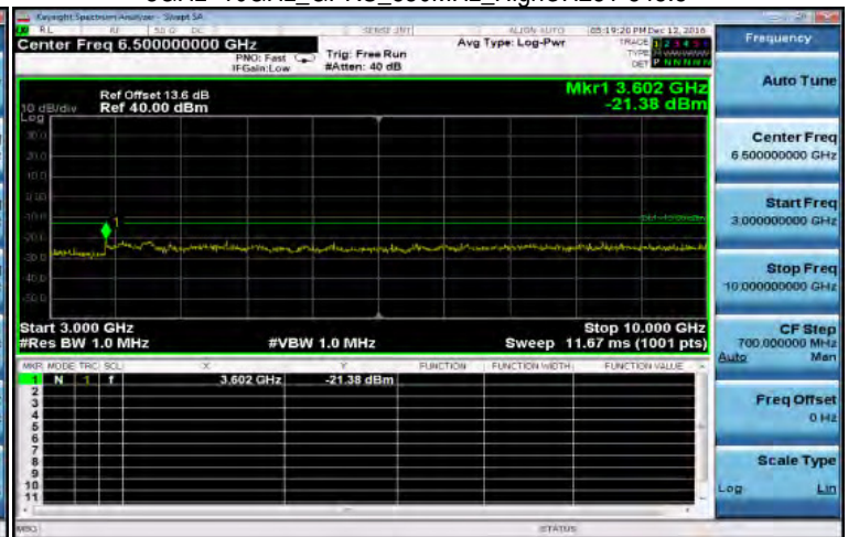
3GHz-10GHz_GPRS_850MHz_HighCH251-848.8
