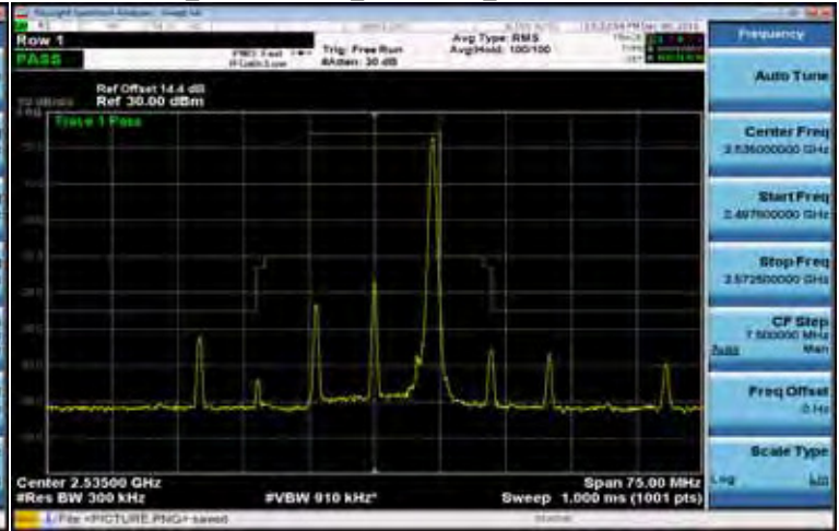
Mask_Band7 15MHz_QPSK 1 74_MidCH20175-2535
