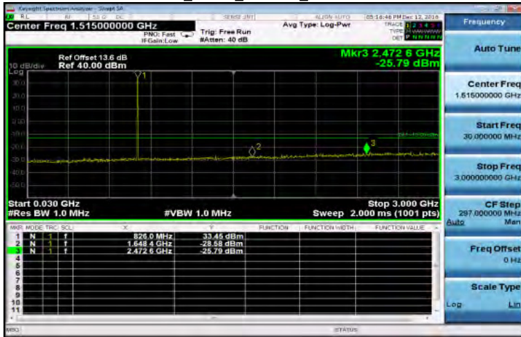
30MHz-3GHz_GPRS_850MHz_LowCH128-824.2
