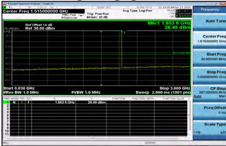
30MHz~3GHz_CDMA2000_BC1_LowCH25-1851.3
