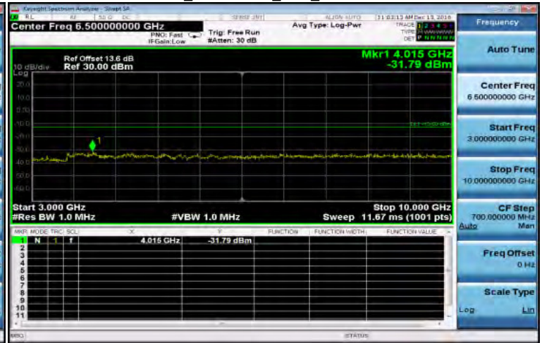
3GHz~10GHz_CDMA2000_BC0_MidCH384-836.52
