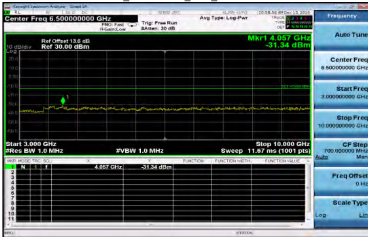
3GHz~10GHz_CDMA2000_BC0_LowCH1013-824.7
