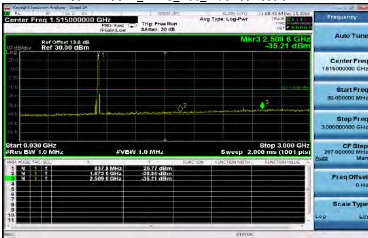
30MHz~3GHz_EVDO_BC0_MidCH384-836.52
