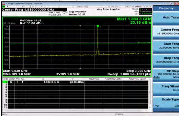
30MHz~3GHz_HSDPA_B2_MidCH9400-1880
