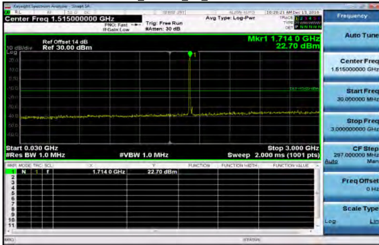
30MHz~3GHz_HSUPA_B4_LowCH1312-1712.4
