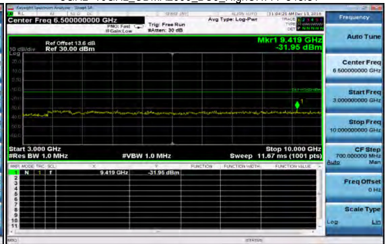
3GHz~10GHz_CDMA2000_BC0_HighCH777-848.31
