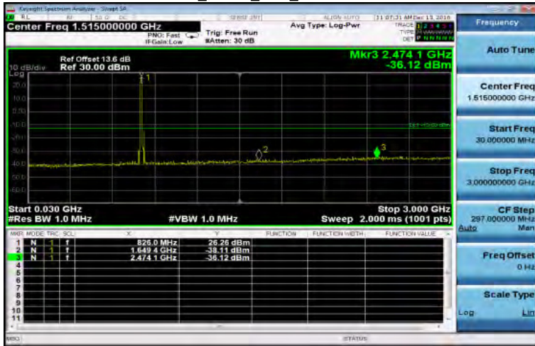
30MHz~3GHz_EVDO_BC0_LowCH1013-824.7
