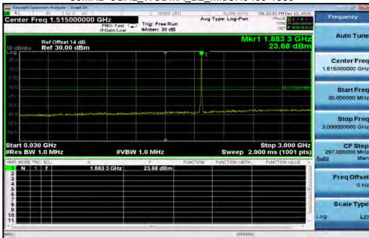
30MHz~3GHz_WCDMA_B2_MidCH9400-1880
