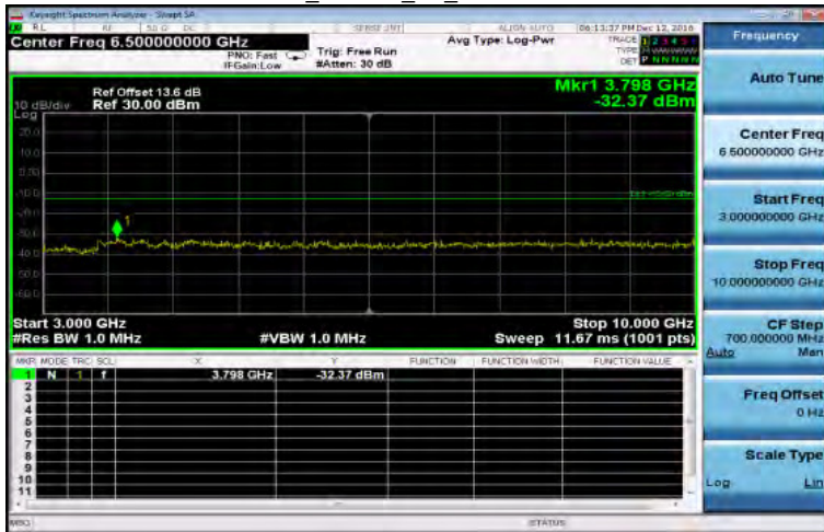
3GHz-10GHz_HSUPA_B5_LowCH4132-826.4
