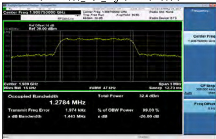
CDMA2000_BC1_HighCH1175-1908.8
