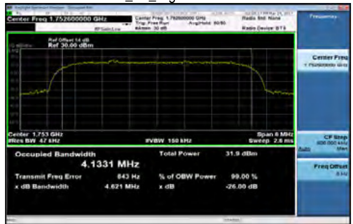
HSUPA_B4_HighCH1513-1752.6
