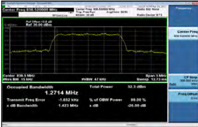
CDMA2000_BC0_MidCH384-836.52
