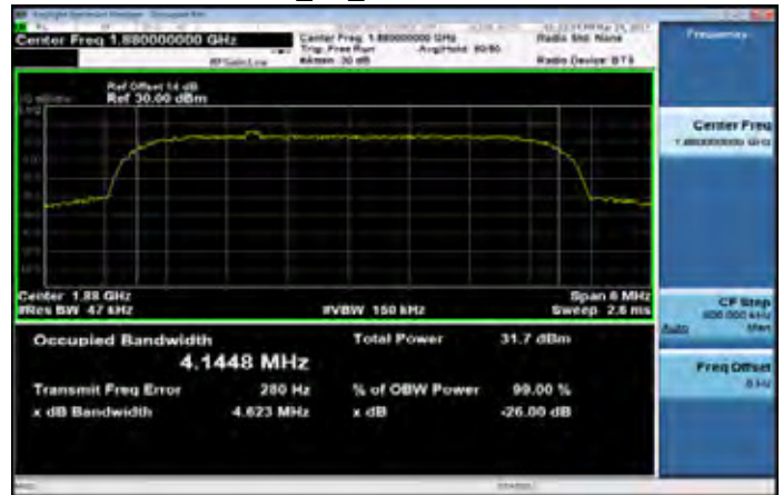
HSDPA_B2_MidCH9400-1880
