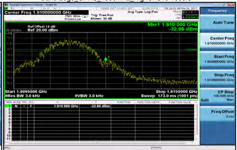
Band Edge_GPRS_1900MHz_HighCH810-1909.8
