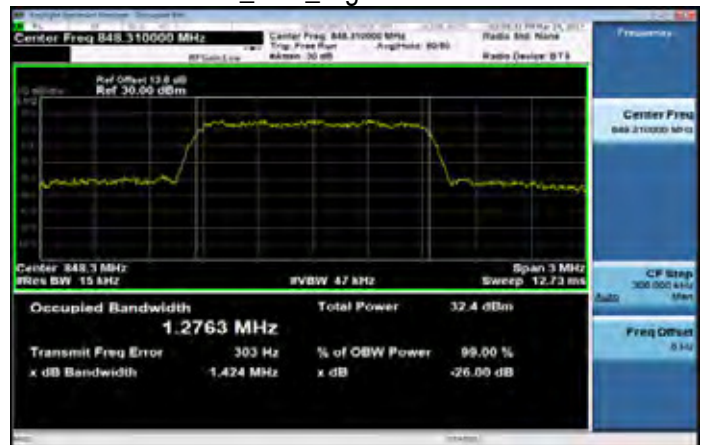
EVDO_BC0_HighCH777-848.31
