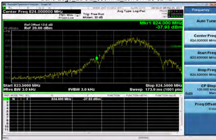
Band Edge_EDGE_850MHz_LowCH128-824.2
