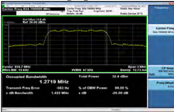
CDMA2000_BC0_LowCH1013-824.7
