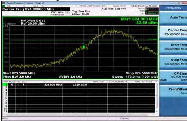
Band Edge_GPRS_850MHz_LowCH128-824.2
