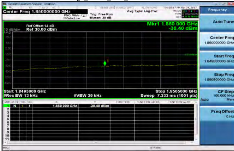
Band Edge_EVDO_BC1_LowCH25-1851.3
