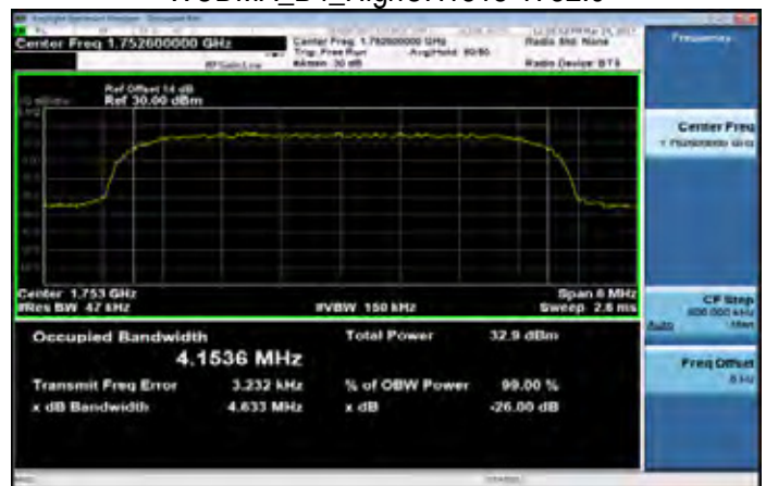
WCDMA_B4_HighCH1513-1752.6
