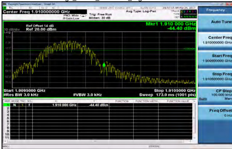
Band Edge_EDGE_1900MHz_HighCH810-1909.8
