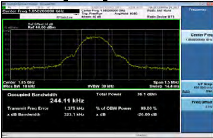
GPRS_1900MHz_LowCH512-1850.2
