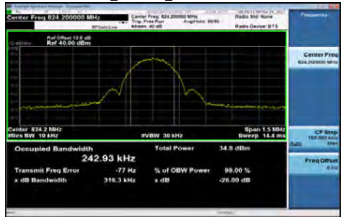
EDGE_850MHz_LowCH128-824.2
