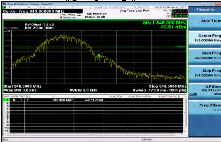
Band Edge_GPRS_850MHz_HighCH251-848.8
