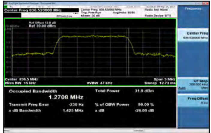
EVDO_BC0_MidCH384-836.52
