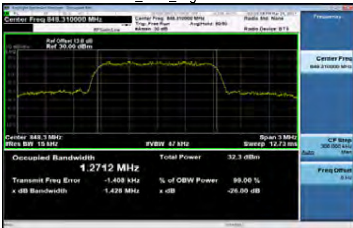
CDMA2000_BC0_HighCH777-848.31
