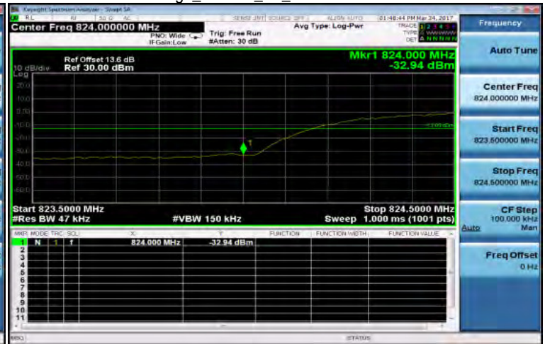
Band Edge_HSUPA_B5_LowCH4132-826.4
