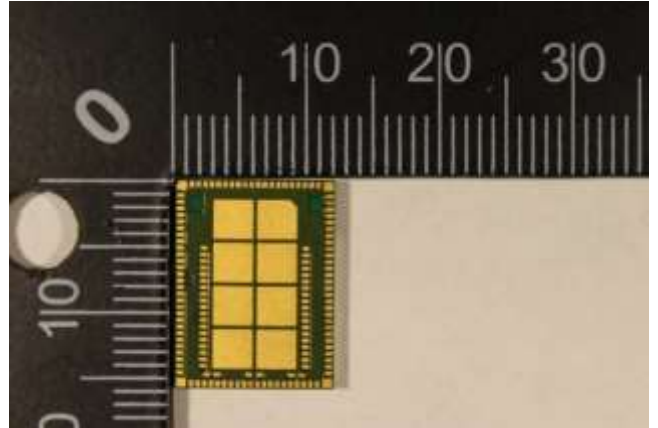
Adapter Back
