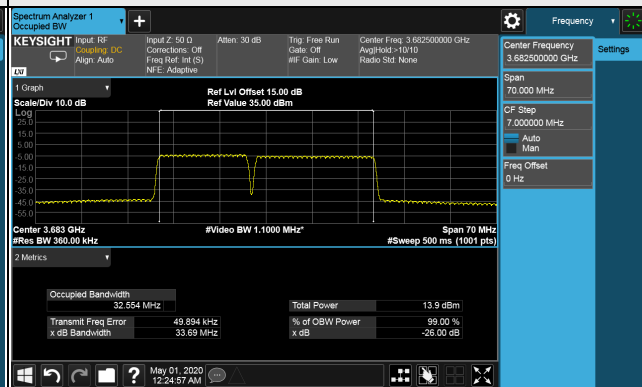
26dB Bandwidth Spectrum Plot of Worst Value 15MHz+20MHz / 256QAM
