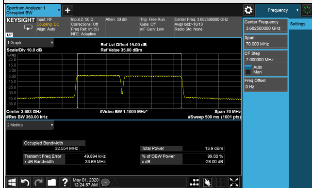
99% Occupied Bandwidth Spectrum Plot of Worst Value 15MHz+20MHz / 256QAM
