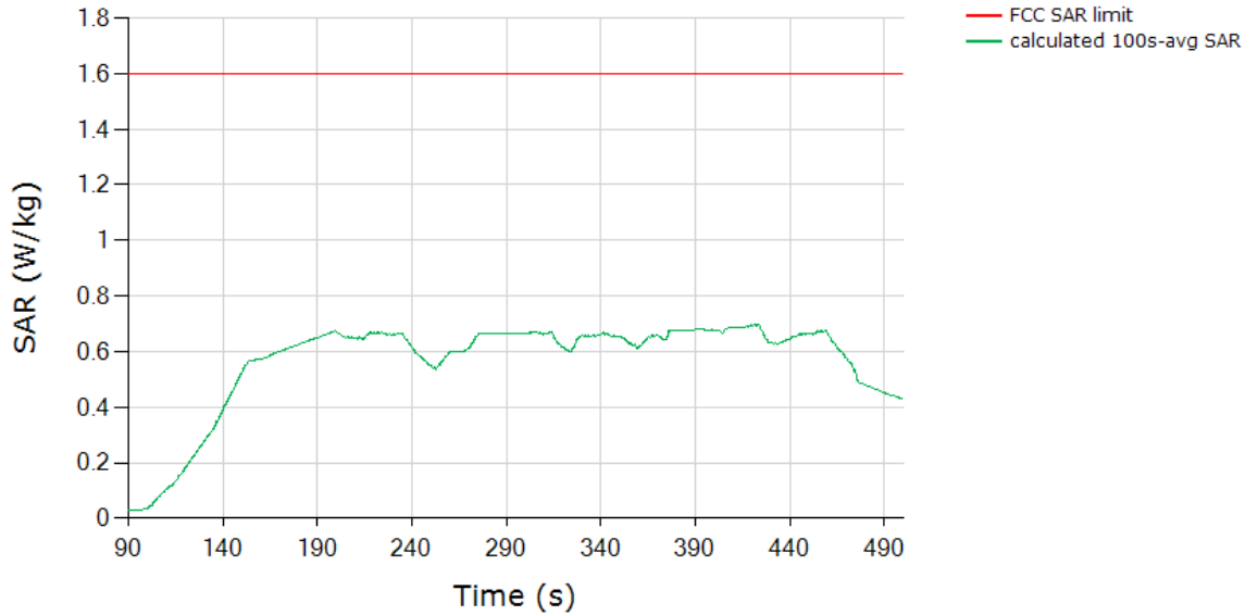
SAR (Test Sequence 2) Tech: NRSUB6, Band n41
