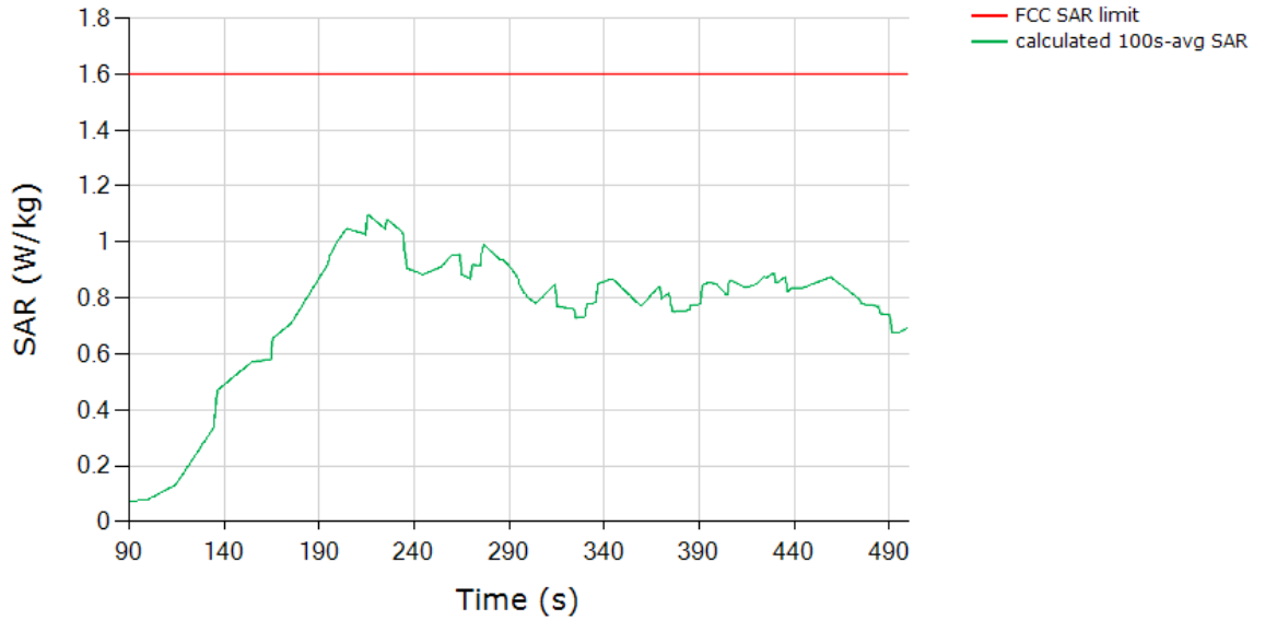
SAR (Test Sequence 2) Tech: LTE, Band 42
