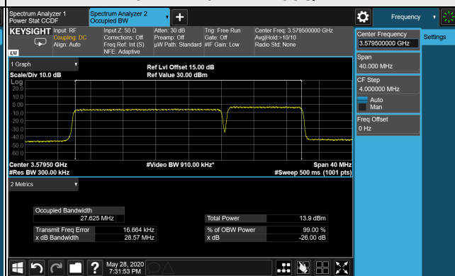
26dB Bandwidth Spectrum Plot of Worst Value 20MHz+10MHz / 256QAM
