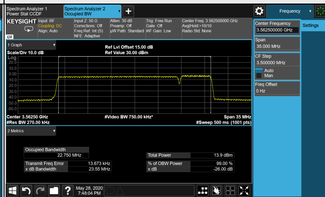
26dB Bandwidth Spectrum Plot of Worst Value 20MHz+5MHz / 256QAM
