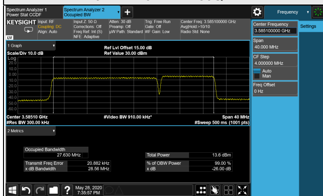
99% Occupied Bandwidth Spectrum Plot of Worst Value 20MHz+10MHz / 256QAM
