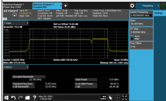
99% Occupied Bandwidth Spectrum Plot of Worst Value 20MHz+5MHz / 256QAM
