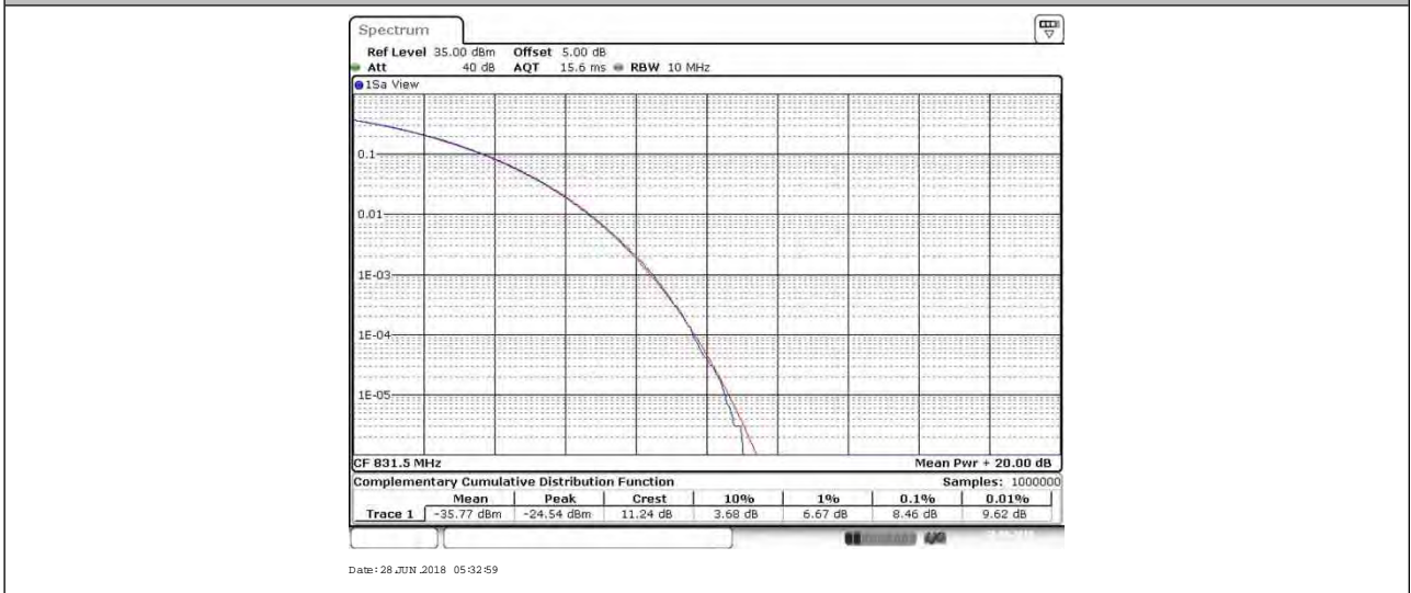
BAND 26_15MHz_64QAM_26915_75RB#0
