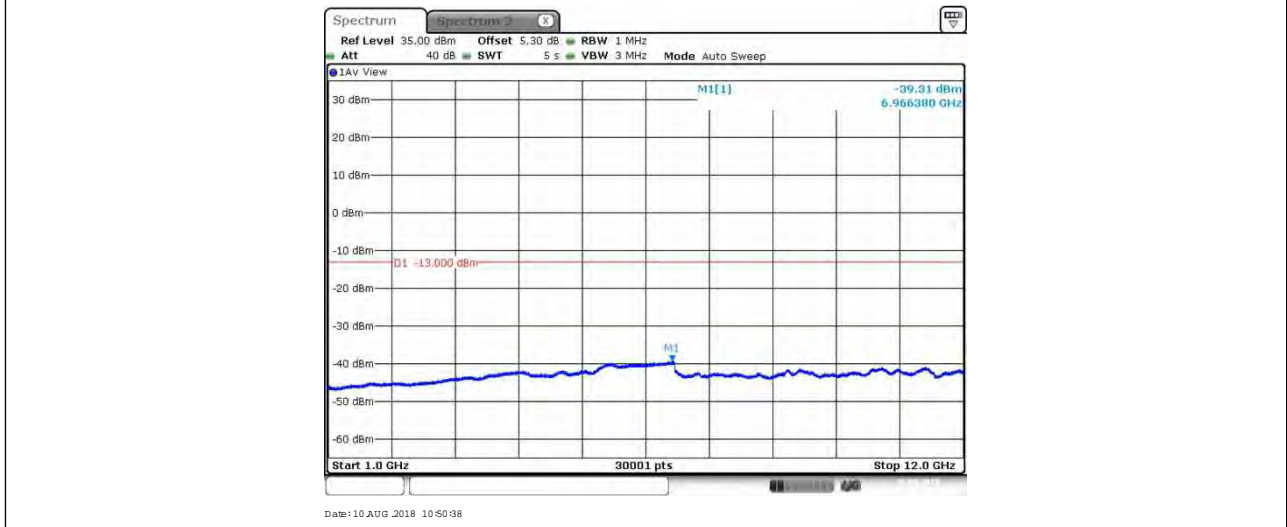
BAND 26_15MHz_16QAM_26915_1RB#0
