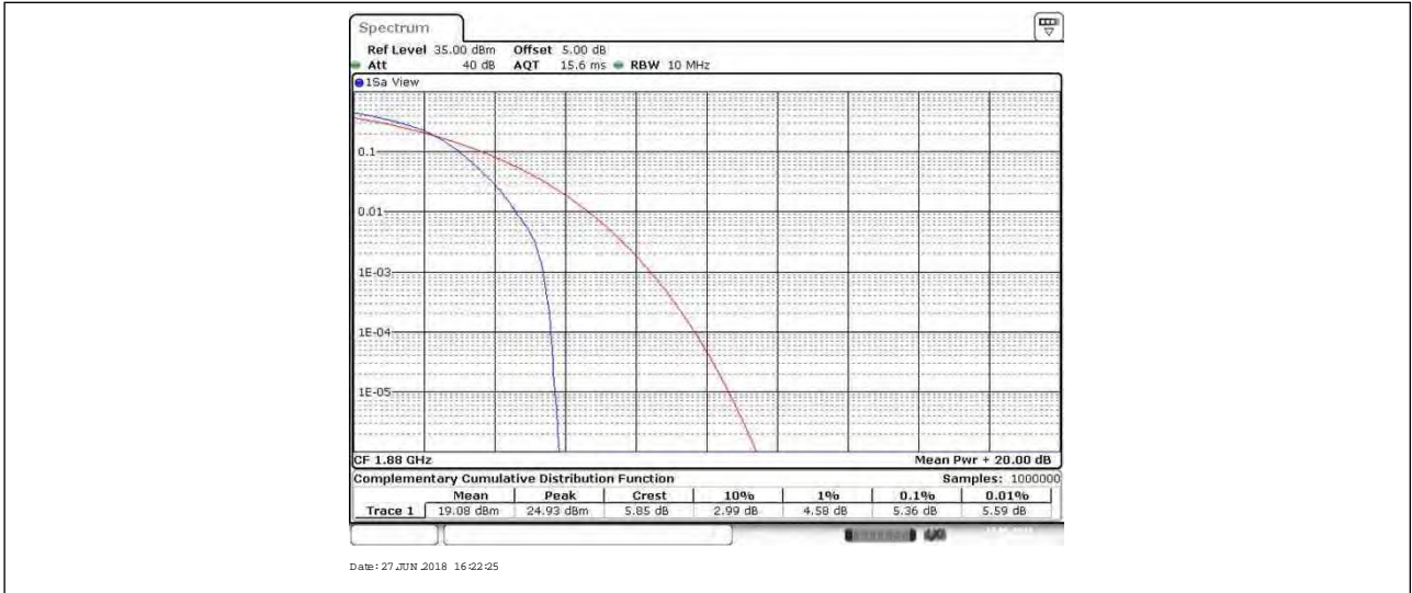
BAND 2_20MHz_16QAM_19100_100RB#0
