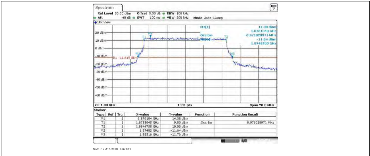
BAND2_10MHz_QPSK_19150_50RB#0
