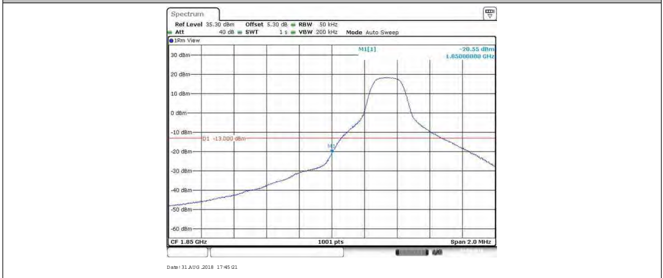
BAND2_5MHz_QPSK_18625_25RB#0
