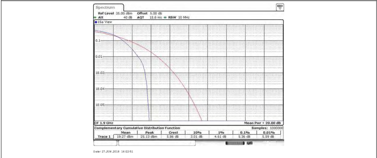
BAND 2_20MHz_64QAM_18700_100RB#0
