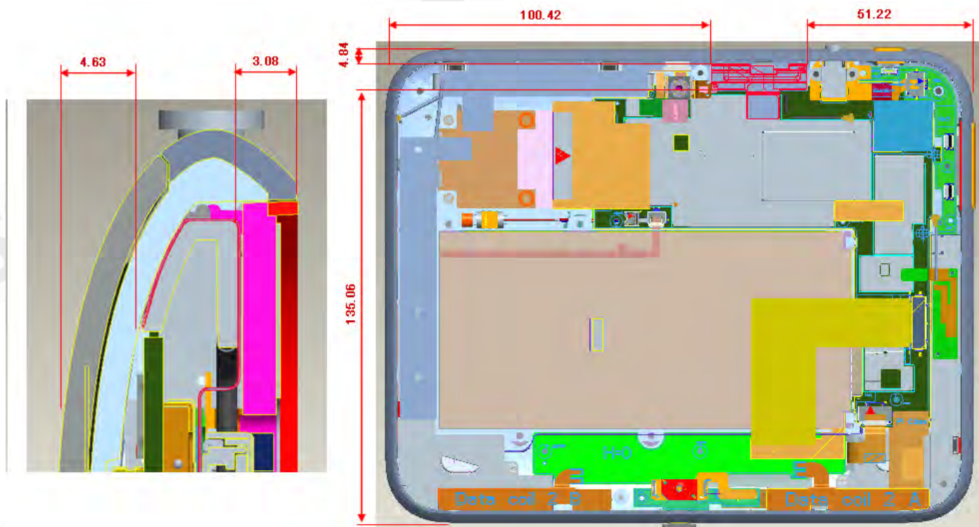
Fig.10 Antenna position of EUT
