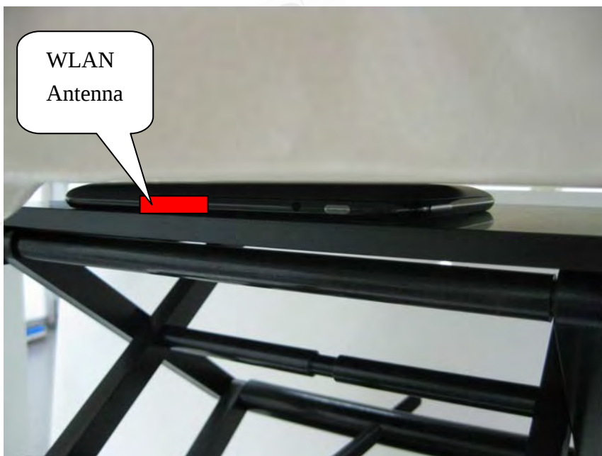
Fig.3 Lap-held mode
