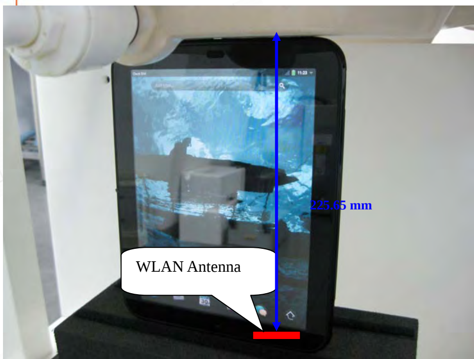
Fig.7 Primary Portrait mode
