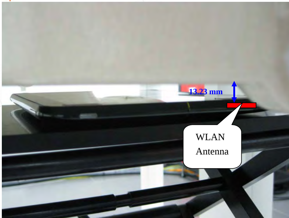
Fig.3 Front side mode (test front position 10mm separation distance)
