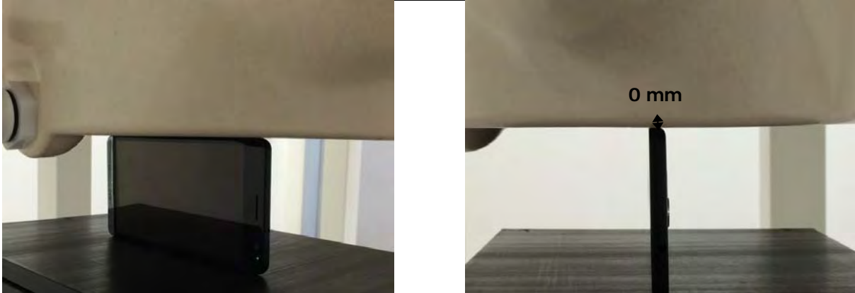
Fig.17 EUT left to flat phantom
