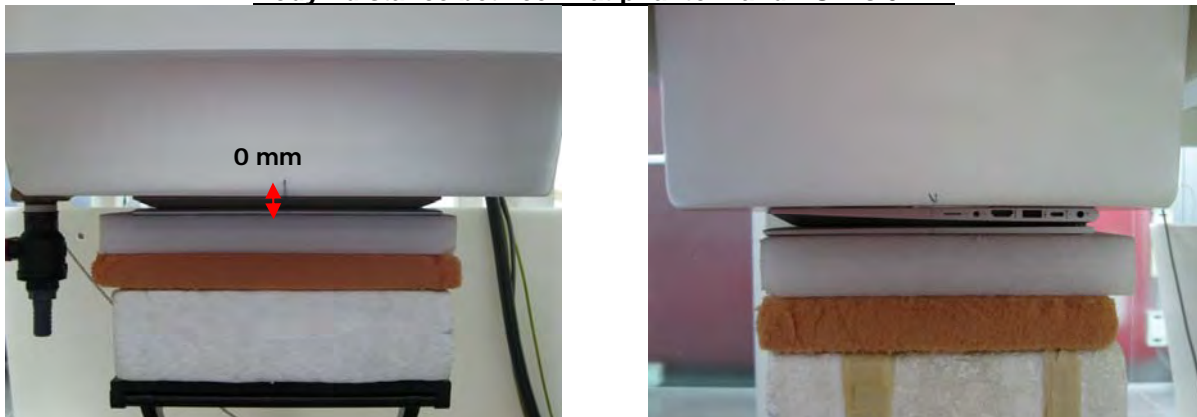
Fig.3 EUT Back side to flat phantom
