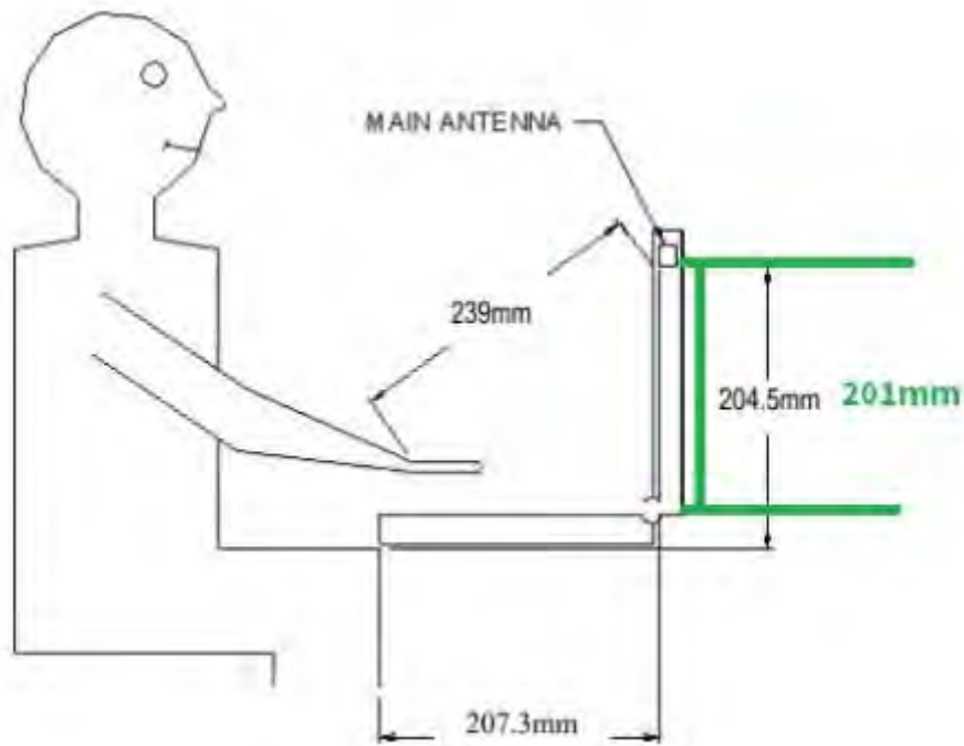
Fig.11 Antenna location of EUT (laptop mode) - End of Report -
