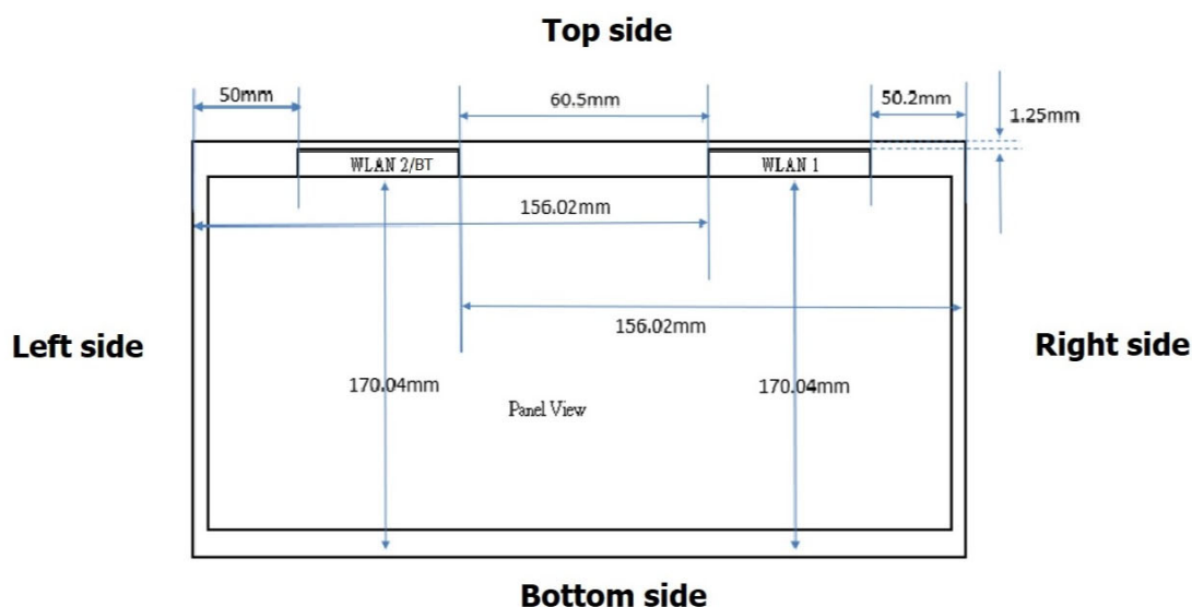
Fig.15 Antenna location of EUT (Tablet mode)
