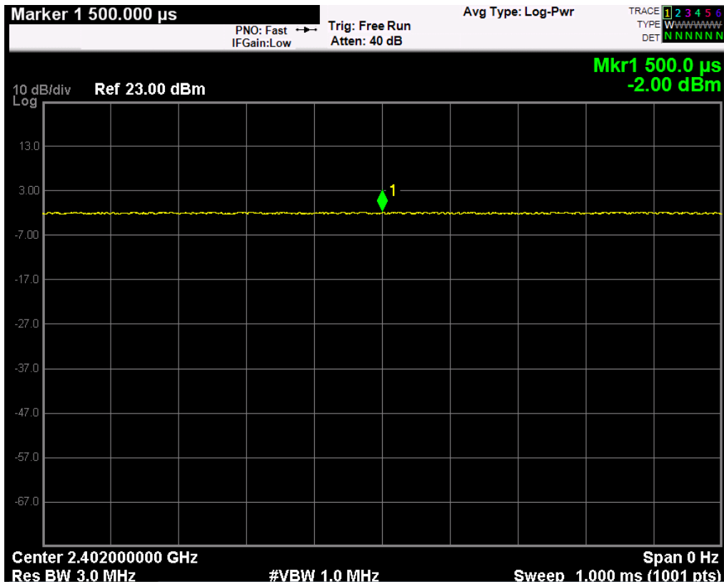
Time-domain plot for Bluetooth transmission signal
