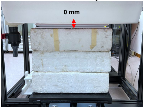
Photograph 1. Body, Back Surface, 0mm (Tablet mode)
