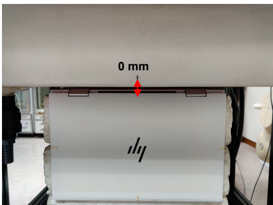
Photograph 11. Body, Bottom Edge, 0mm (Laptop mode)
