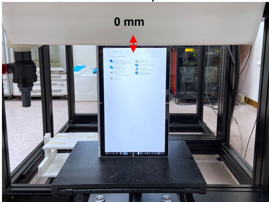
Photograph 9. Body, Left Edge, 0mm (Tablet mode)
