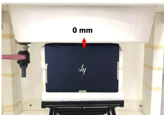
Fig.8 EUT Bottom side (Laptop mode) to flat phantom
