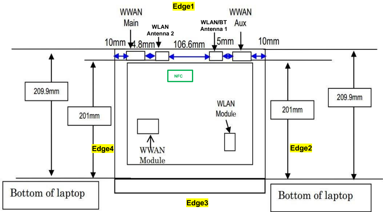
Front View
