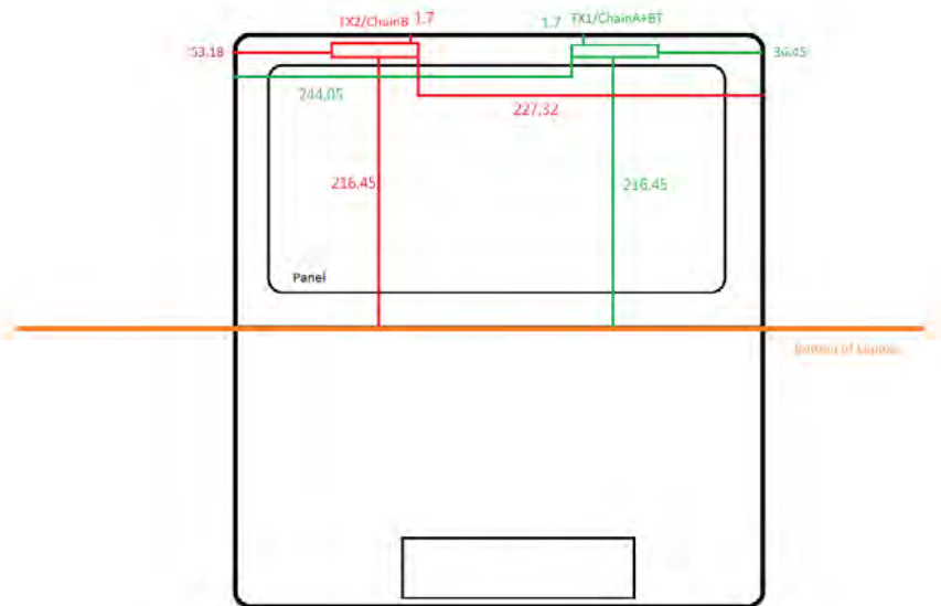
Fig.10 Antenna location of EUT
