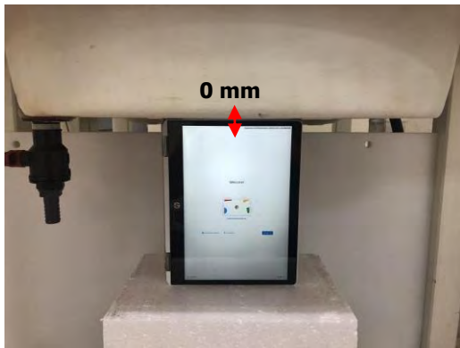
Fig.7 EUT Left side to flat phantom
