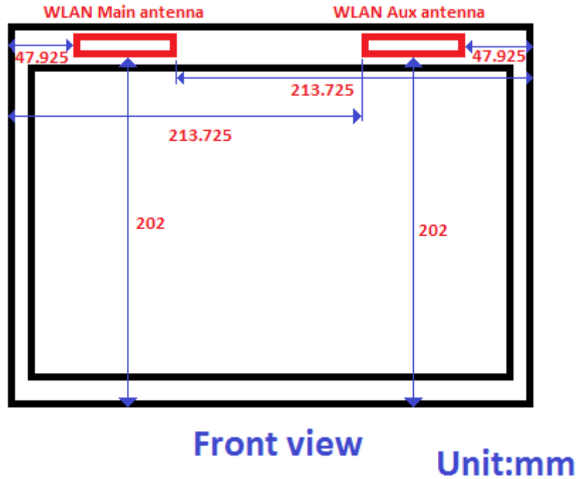
Fig.10 Antenna location of EUT (tablet mode)
