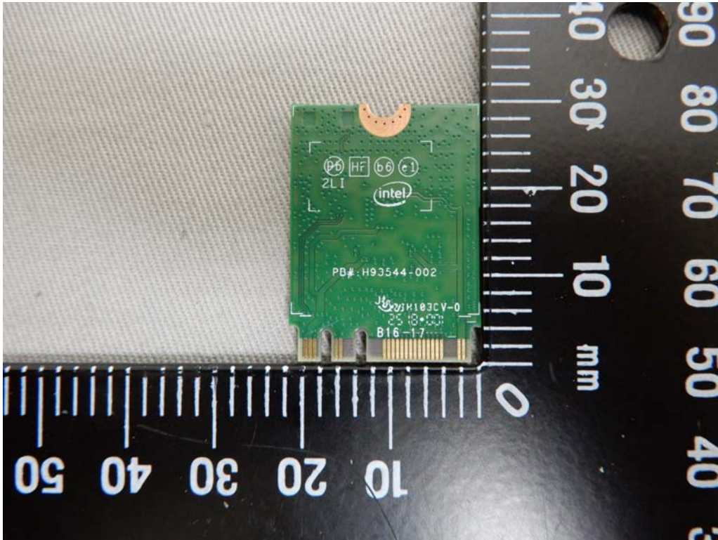
WLAN / BT Module – 3 (Model No.: 8265NGW)
