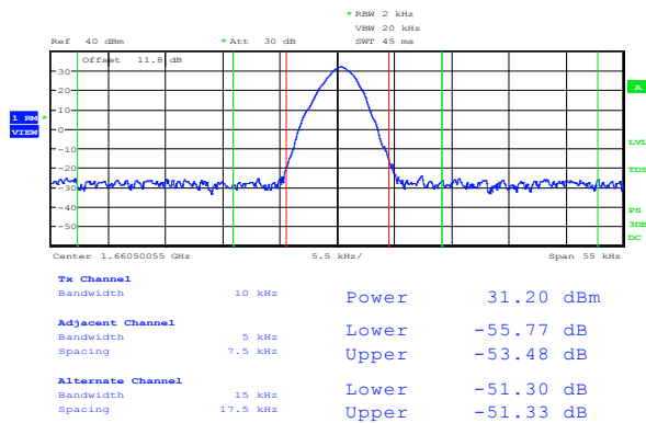
Plot 8.3-3: Emission mask for IDP-680, high channel
