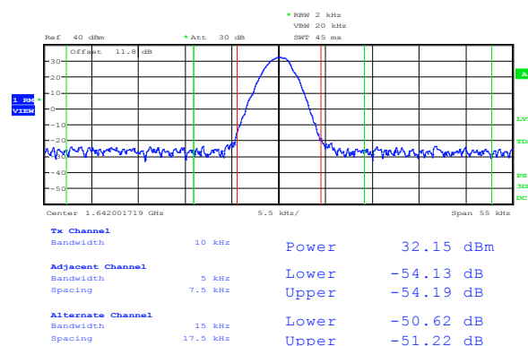
Plot 8.3-5: Emission mask for IDP-690, mid channel
