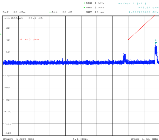
Plot 8.5-3: 1559–1610 MHz for IDP-680, high channel
