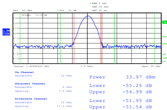
Plot 8.3-1: Emission mask for IDP-680, low channel
