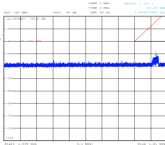
Plot 8.5-4: 1559–1610 MHz for IDP-690, low channel
