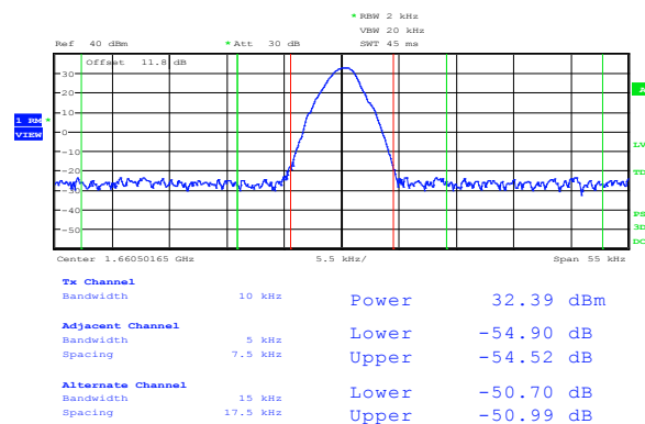
Plot 8.3-6: Emission mask for IDP-690, high channel
