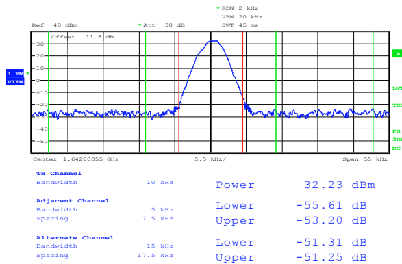
Plot 8.3-2: Emission mask for IDP-680, mid channel
