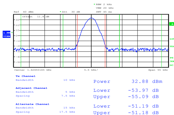
Plot 8.3-4: Emission mask for IDP-690, low channel
