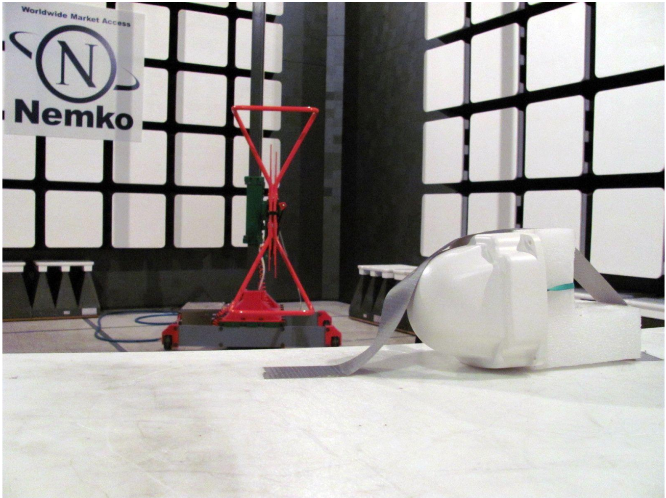
Photo 10.2-2: IDP-690 test setup
