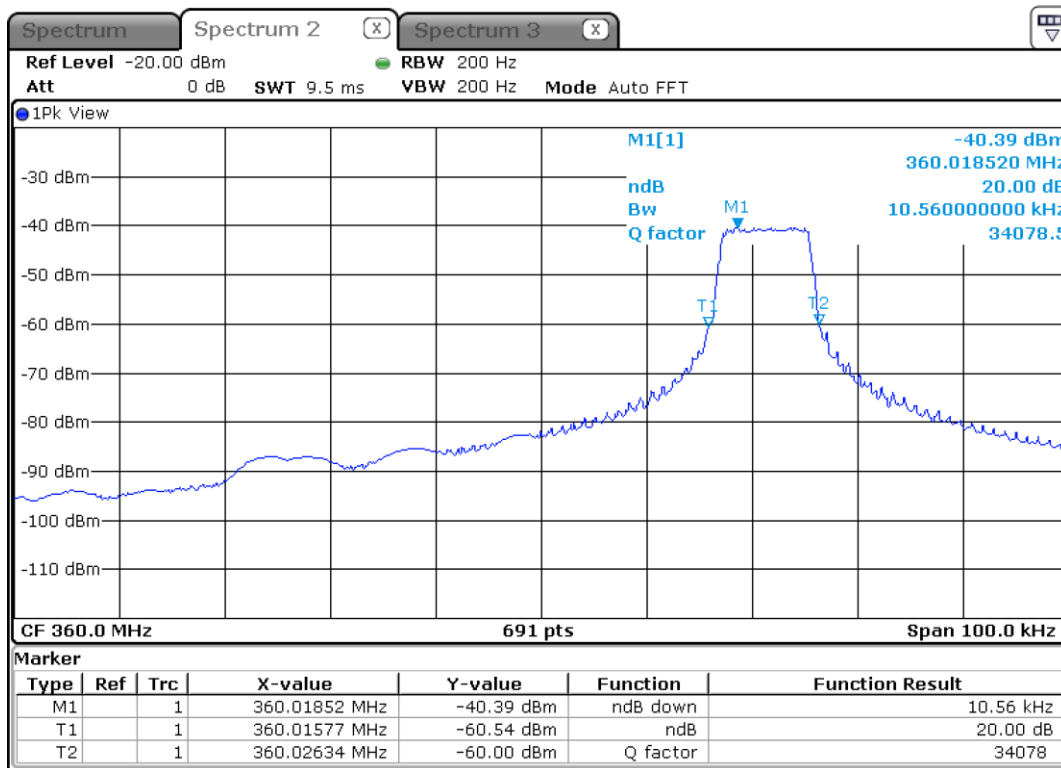
Figure 8.4-1: 20 dB bandwidth, OHD Genie, 9 switch/ 3 position dipswitch, 360 MHz.
