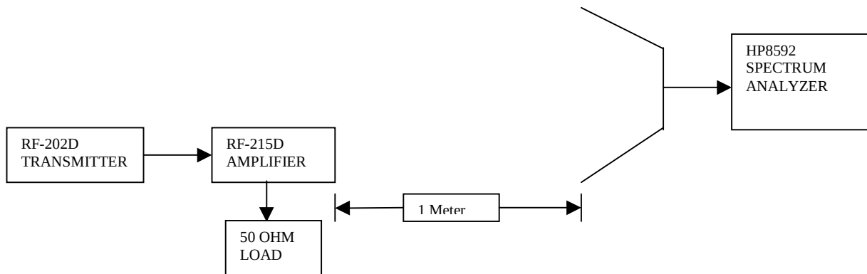
FIGURE 2 – FIELD STRENGTH OF SPURIOUS RADIATION TEST SET-UP
