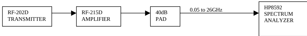
FIGURE 1 – SPURIOUS EMISSION AT ANTENNA TEST SET-UP
