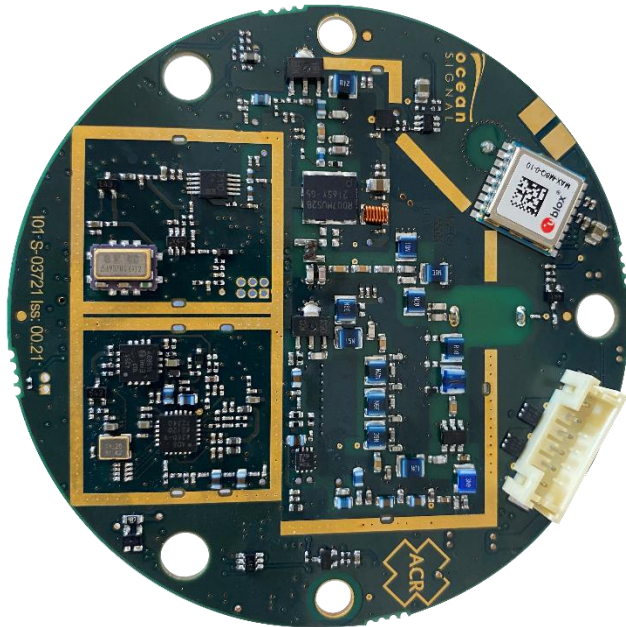
Figure 5: GlobalFix V5 PCB – Rear side with screening cans removed.
