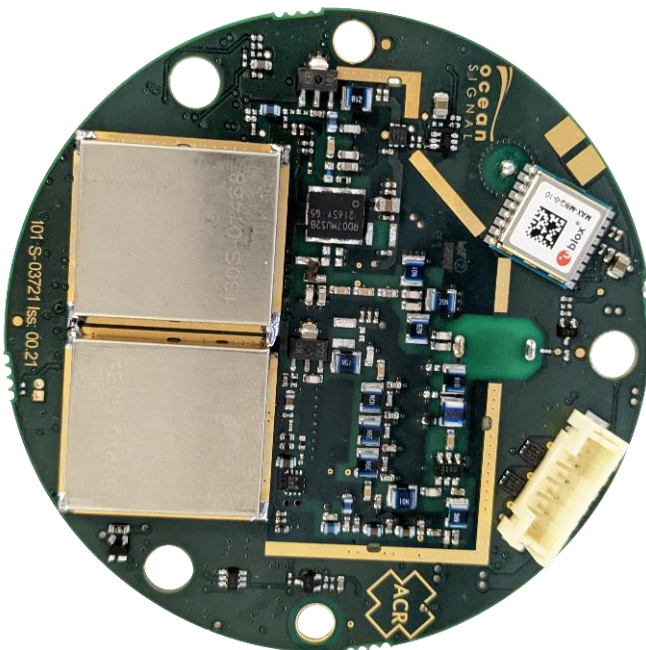
Figure 4: GlobalFix V5 PCB – Rear side
