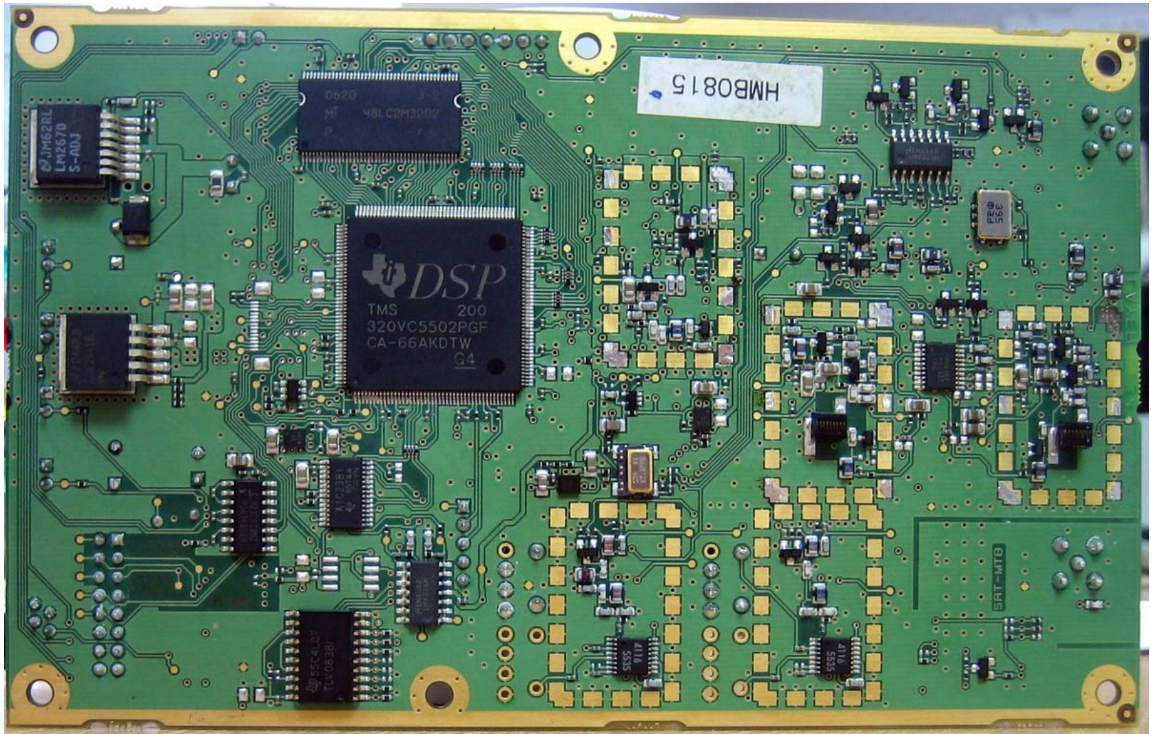
AIS-300 Internal Photos: PCB Bottom
