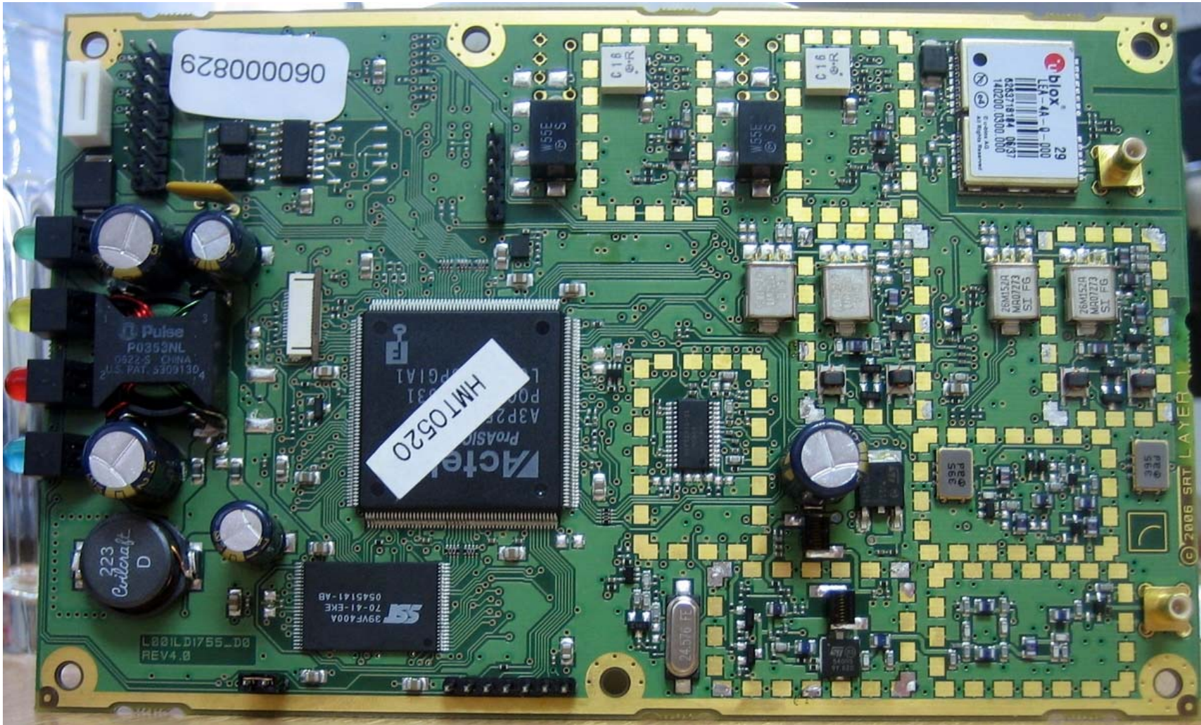
AIS-300 Internal Photos: PCB Top
