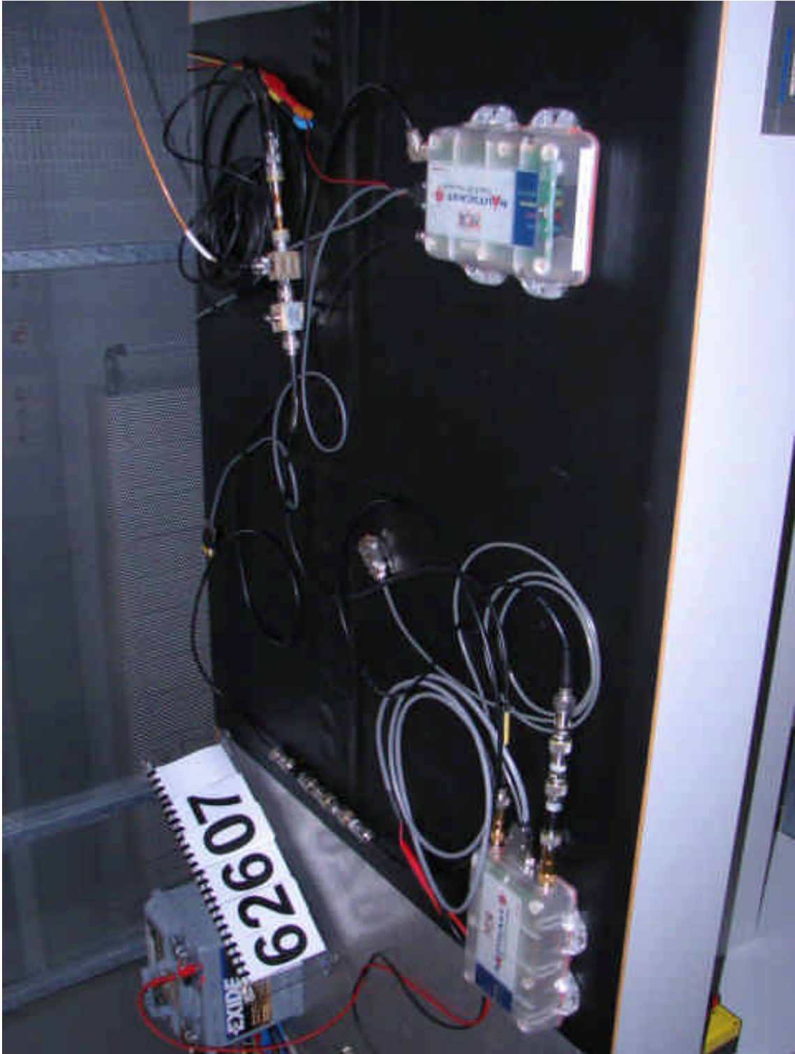
esd5.JPG: Testsetup electrostatic discharge
