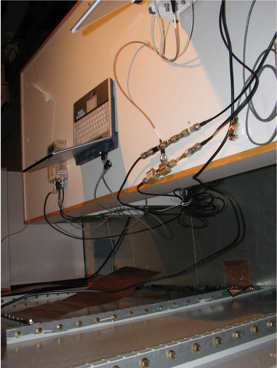
emicon1.JPG: Testsetup conducted emission measurement on DC-line
