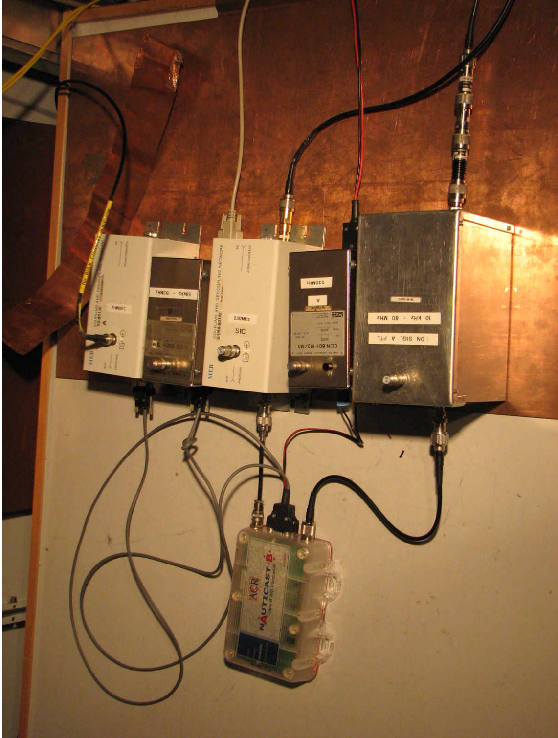
emscon3.JPG: Testsetup conducted high-frequency interference
