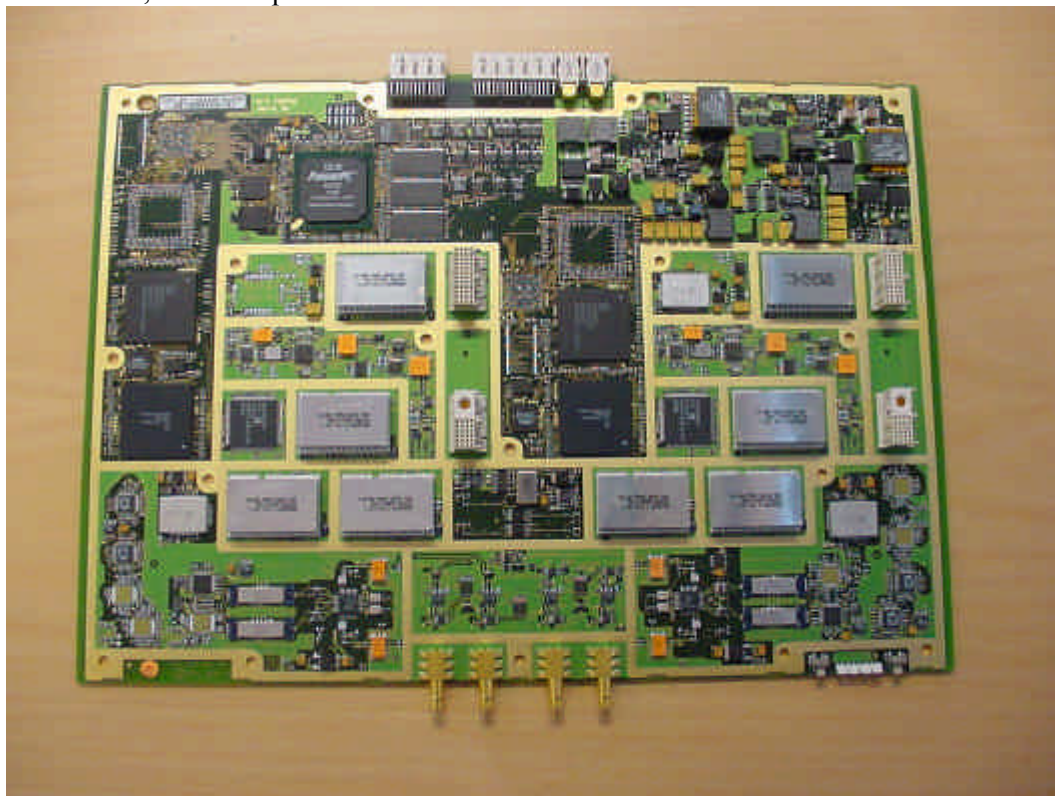
Main board, PCB component side
