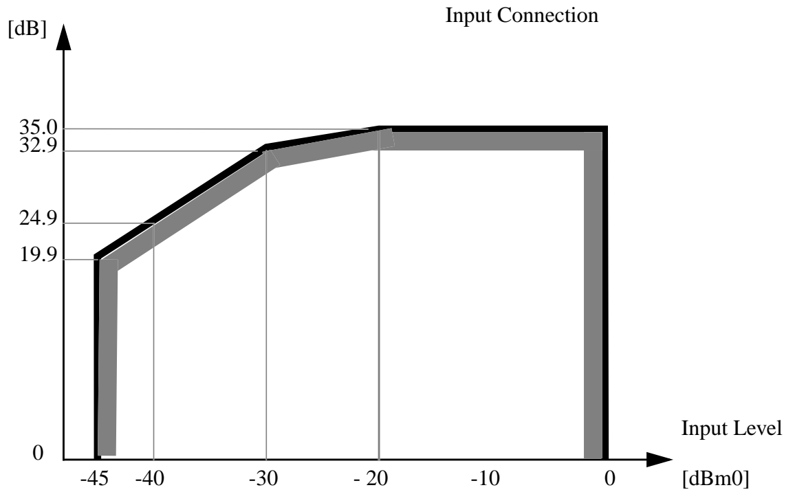
Figure 11. Limits for signal to total distortion ratio as a function of input level. Sine wave method. Input relative level, L_i = 0 dBr
