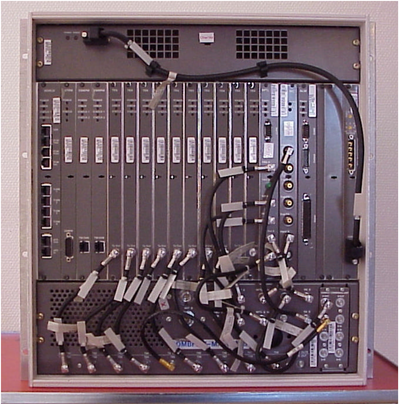
2.1033 (C)(12) Front of RBS884M Micro with DC Supply
