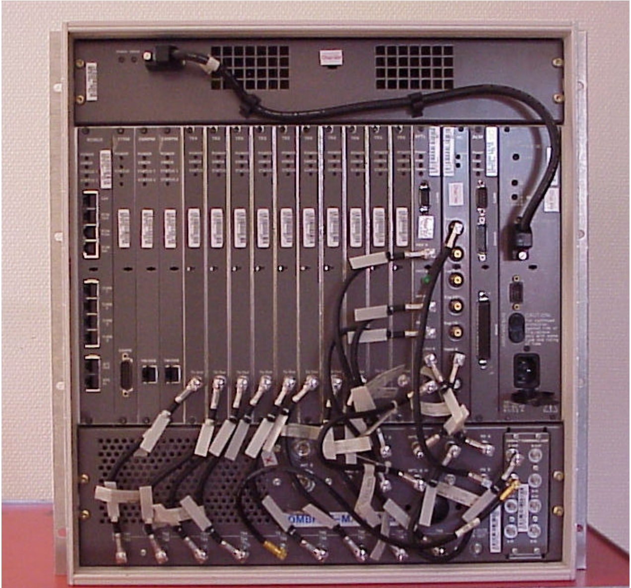
2.1033 (C)(12) Front of RBS884M Micro with AC Supply
