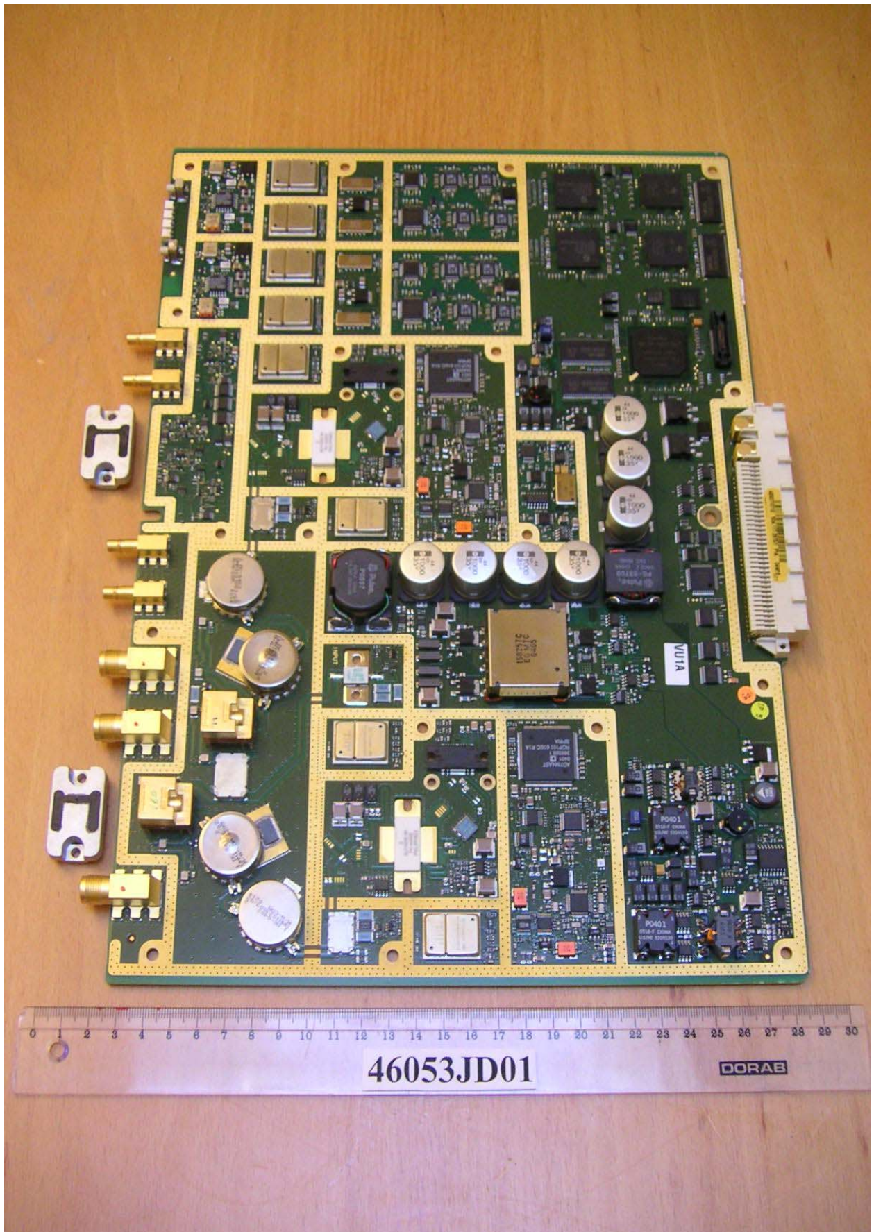
Top view of dTRU-19 PCB
