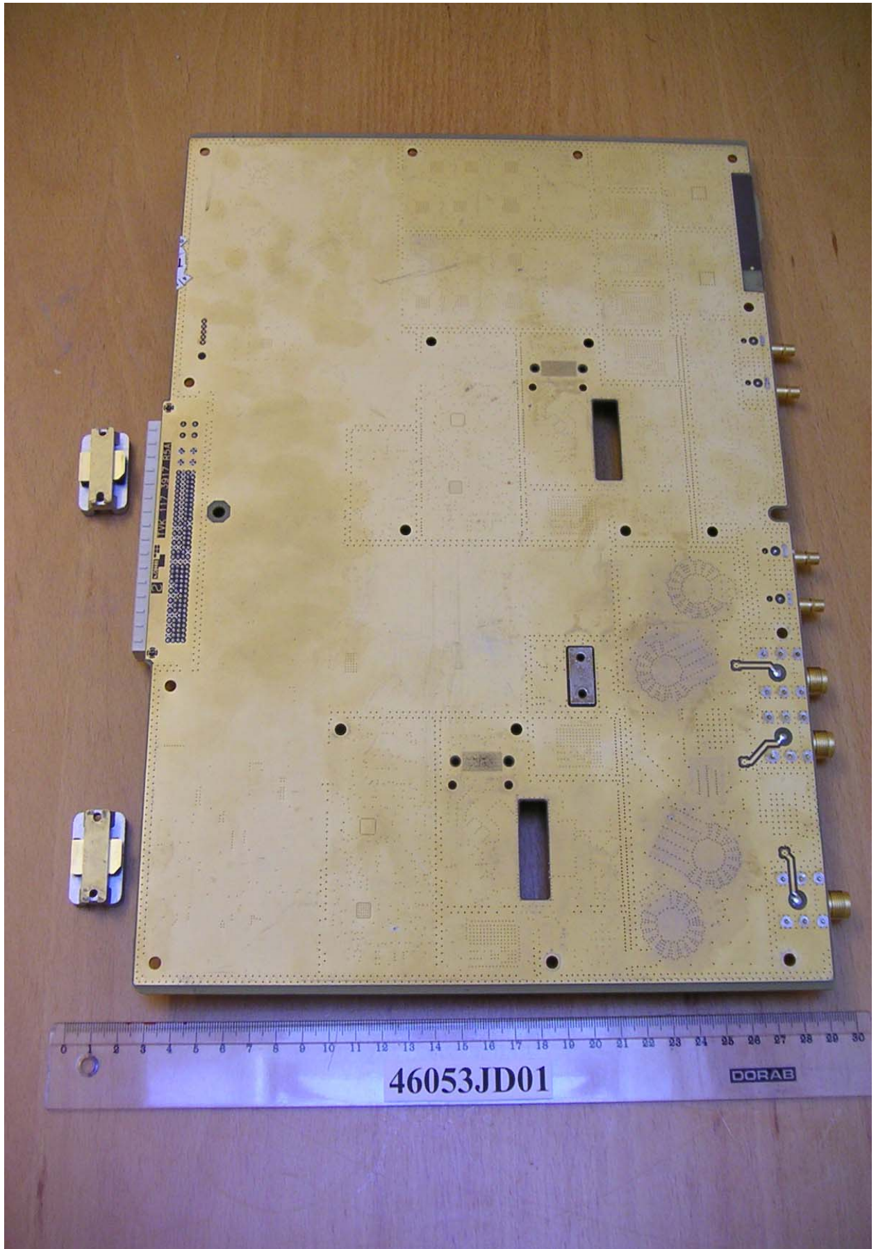
Bottom view of dTRU-19 PCB
