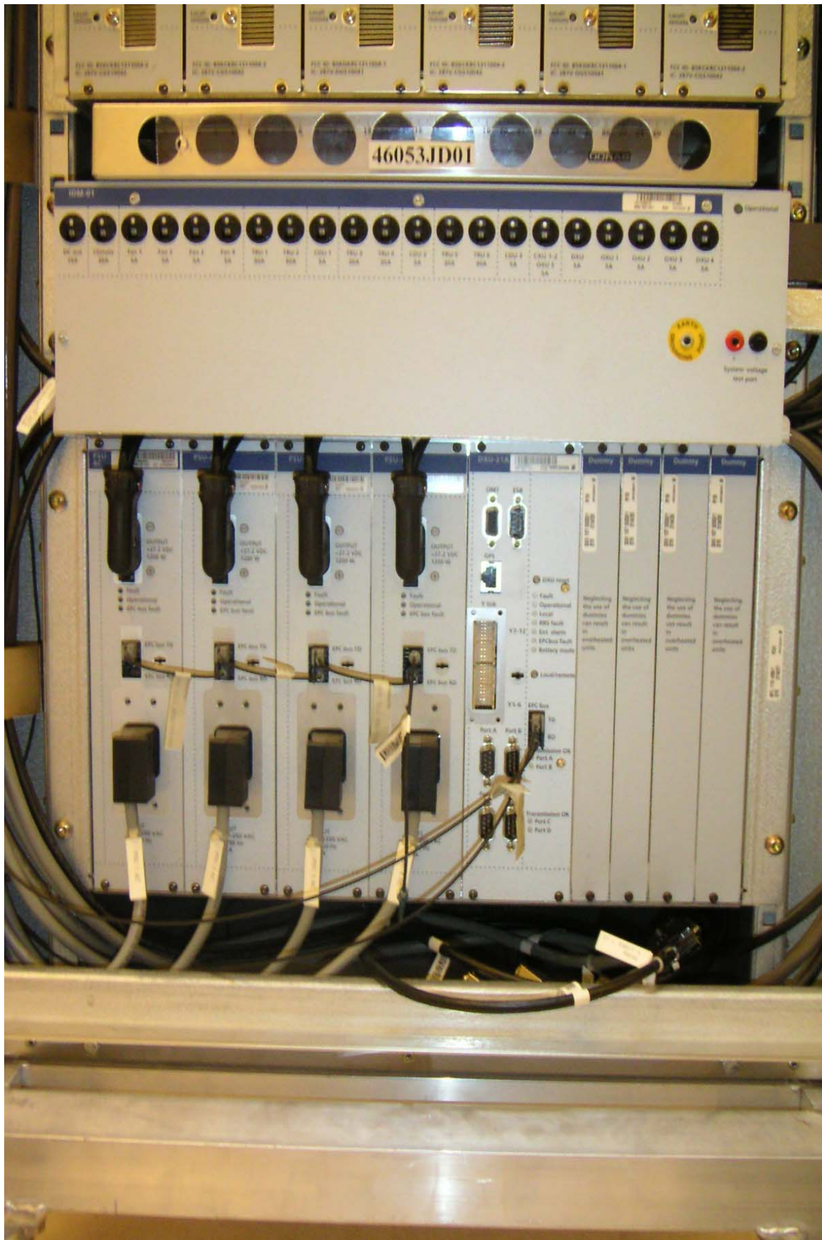
Power Supply/DXU 21-A/IDM-01 shelf view
