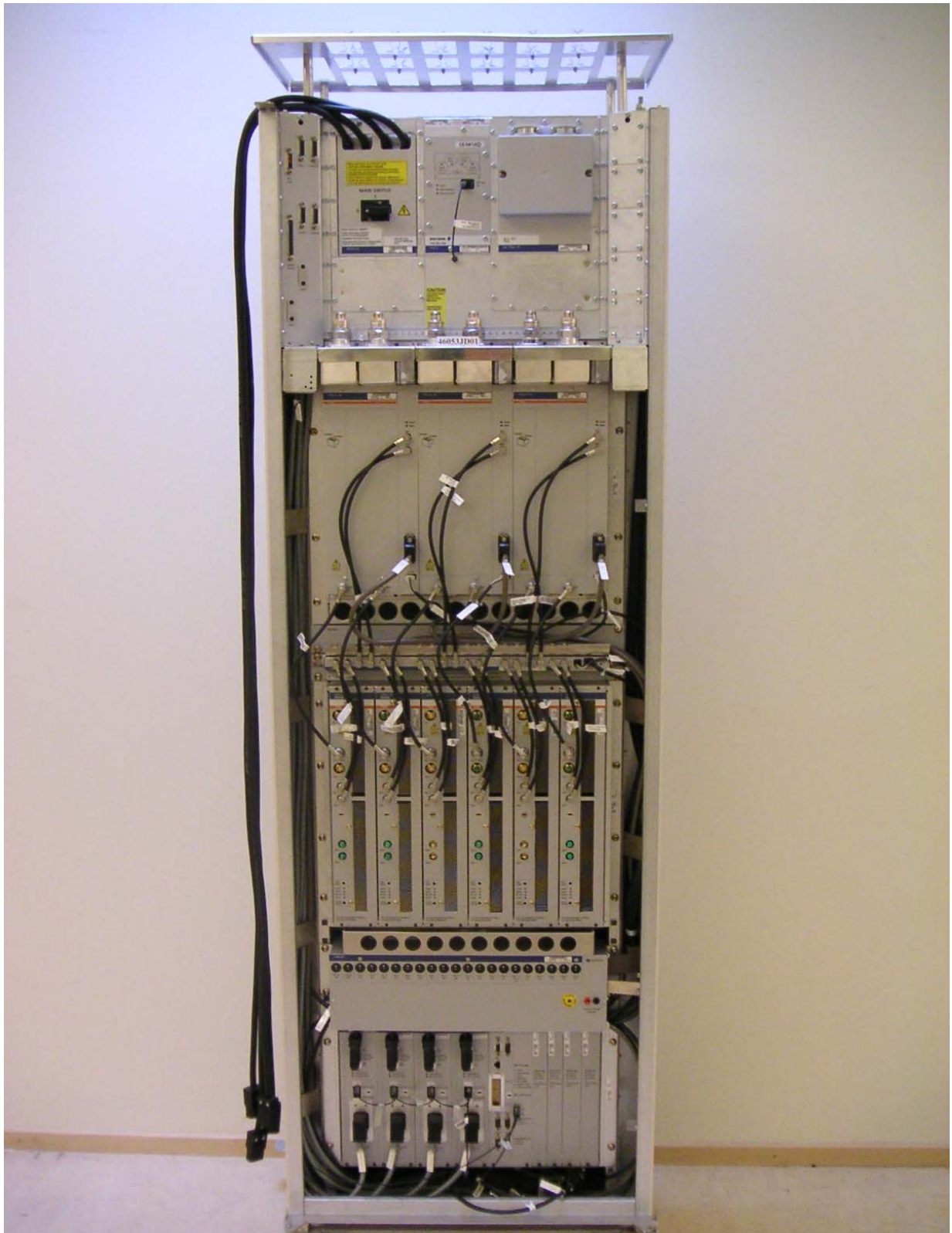
Front view of RBS 2206 GSM 1900 Cabinet
