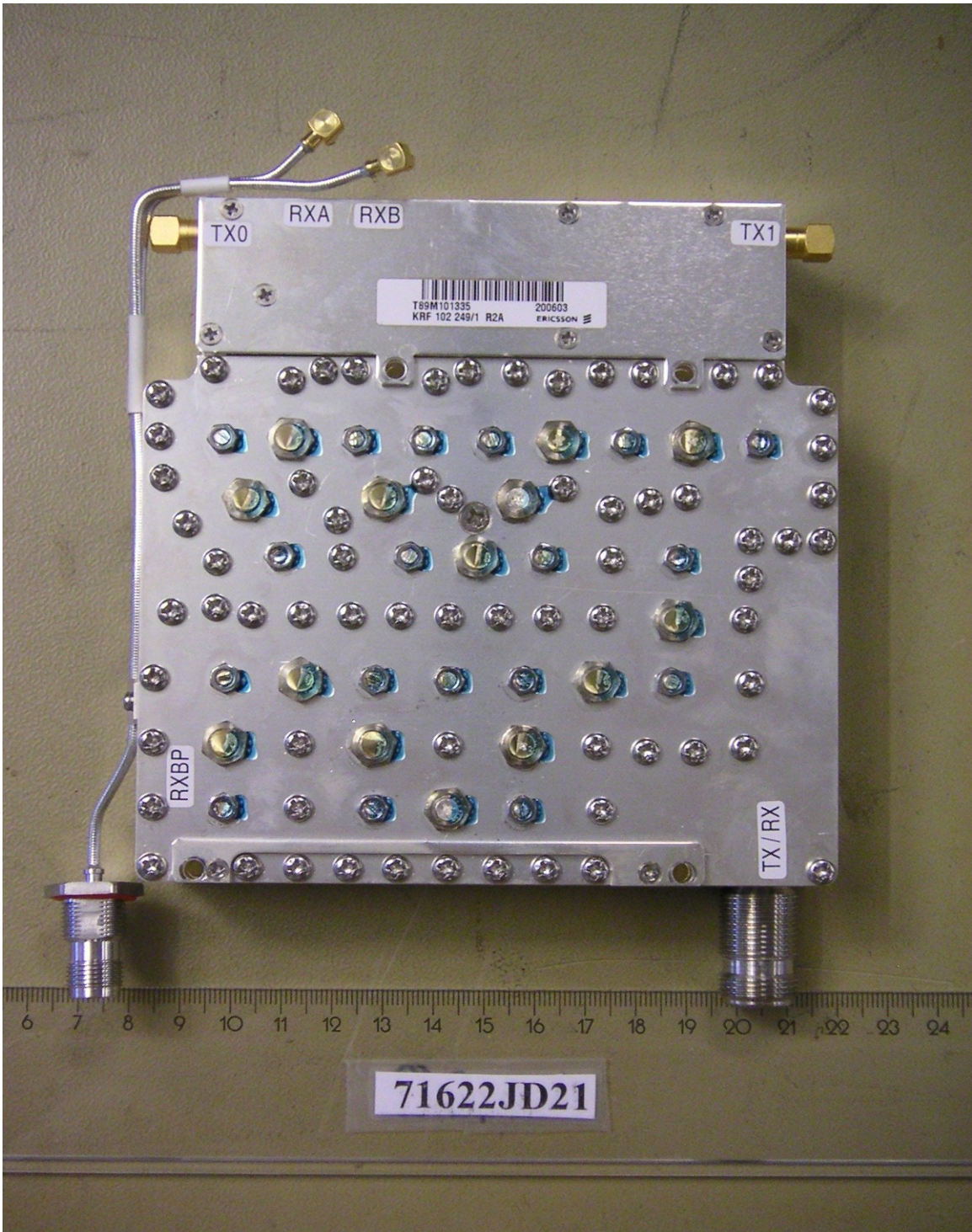
PHT/71622JD21/017 Duplex Filter 1. Front View
