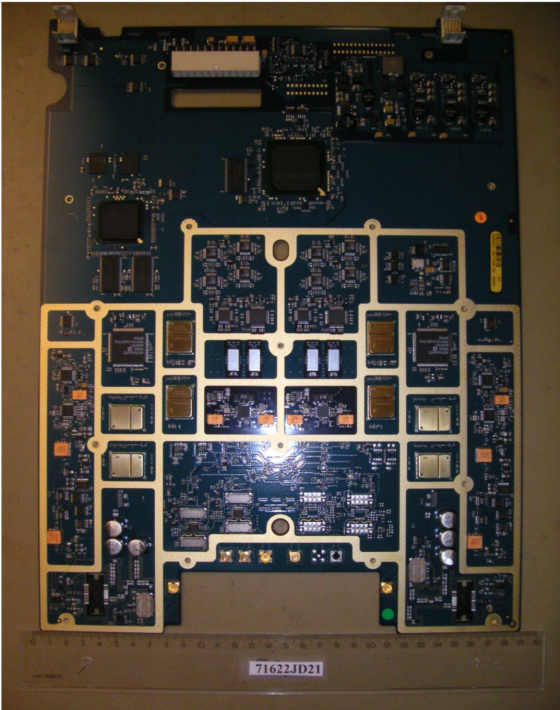
PHT/71622JD21/013 Digital Radio Access Board 1. Front View
