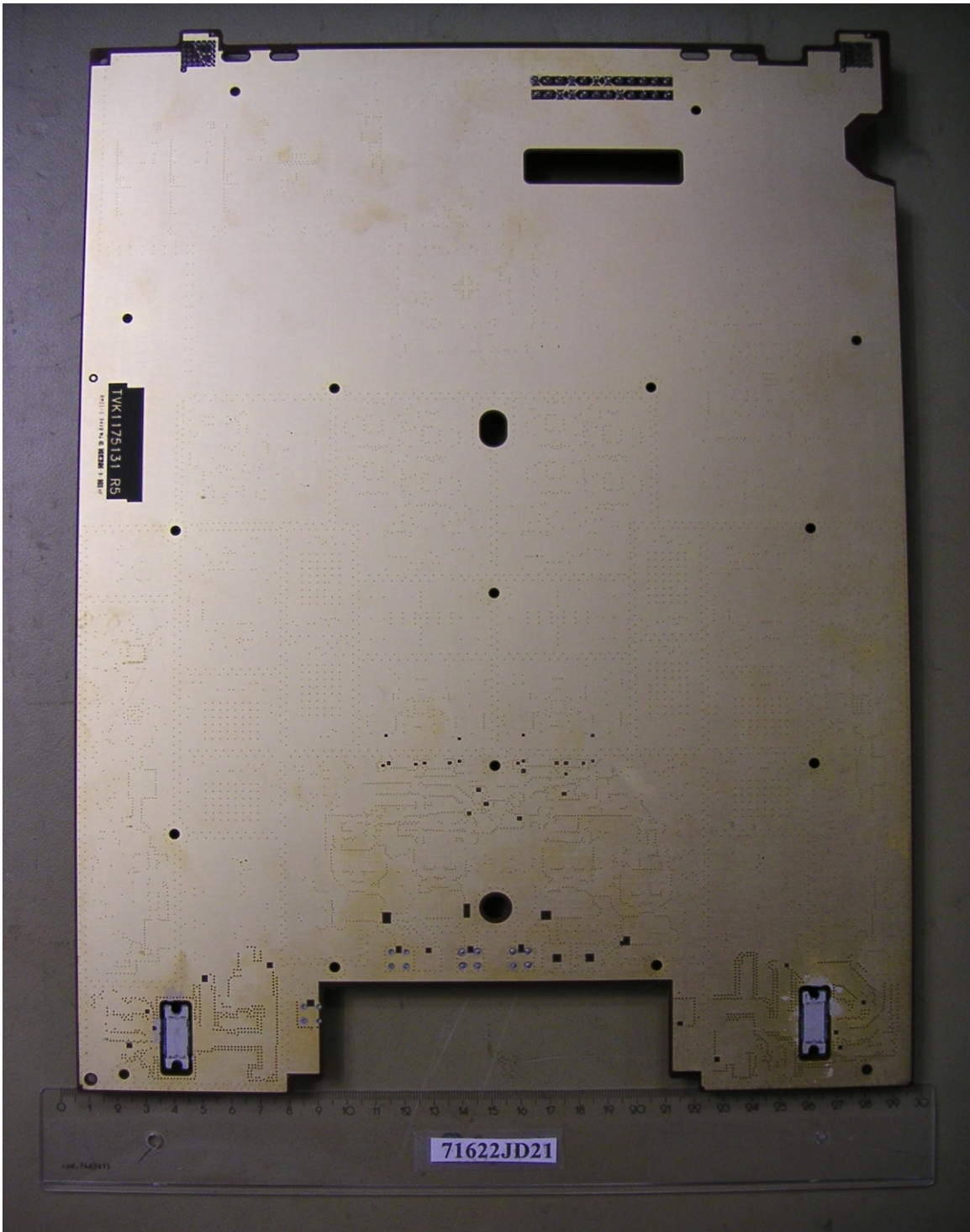
PHT/71622JD21/014 Digital Radio Access Board 1. Back View
