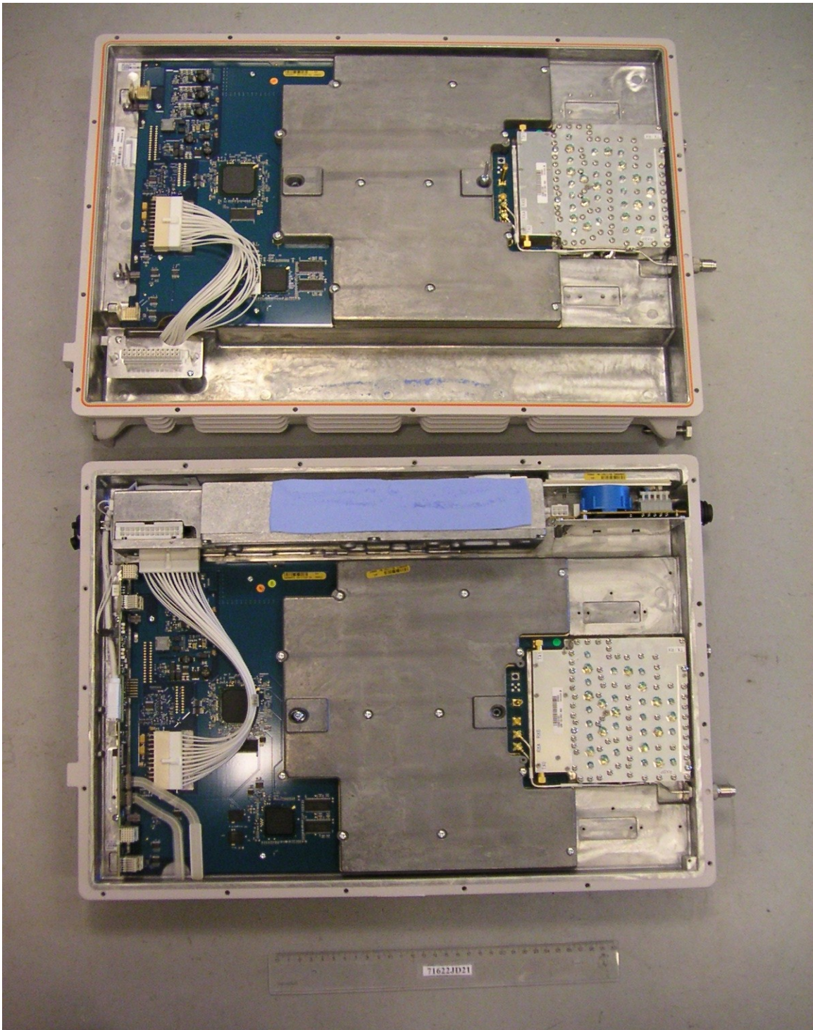
PHT/71622JD21/012 RRU-M8 EDGE. Open View
