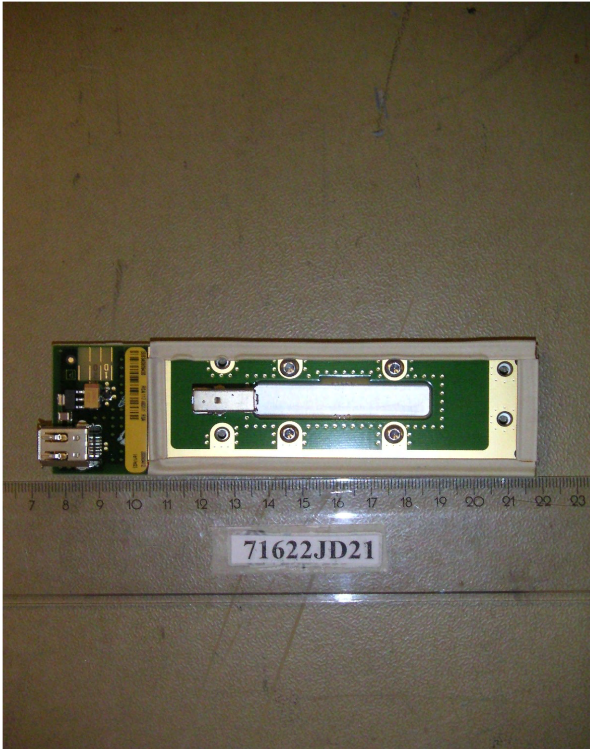
PHT/71622JD21/026 Y Interface Board. Front View
