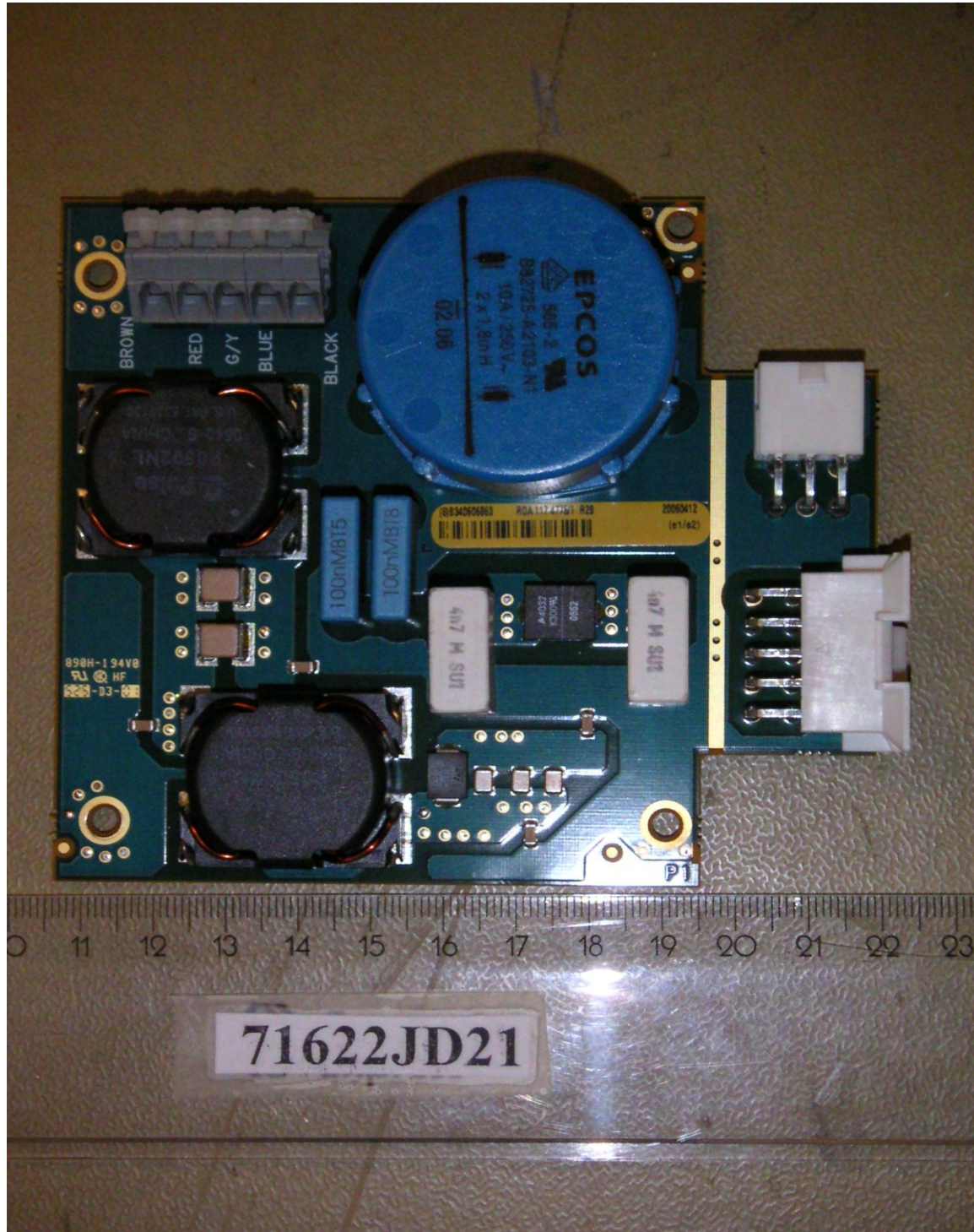
PHT/71622JD21/028 Power Interface Board. Front View
