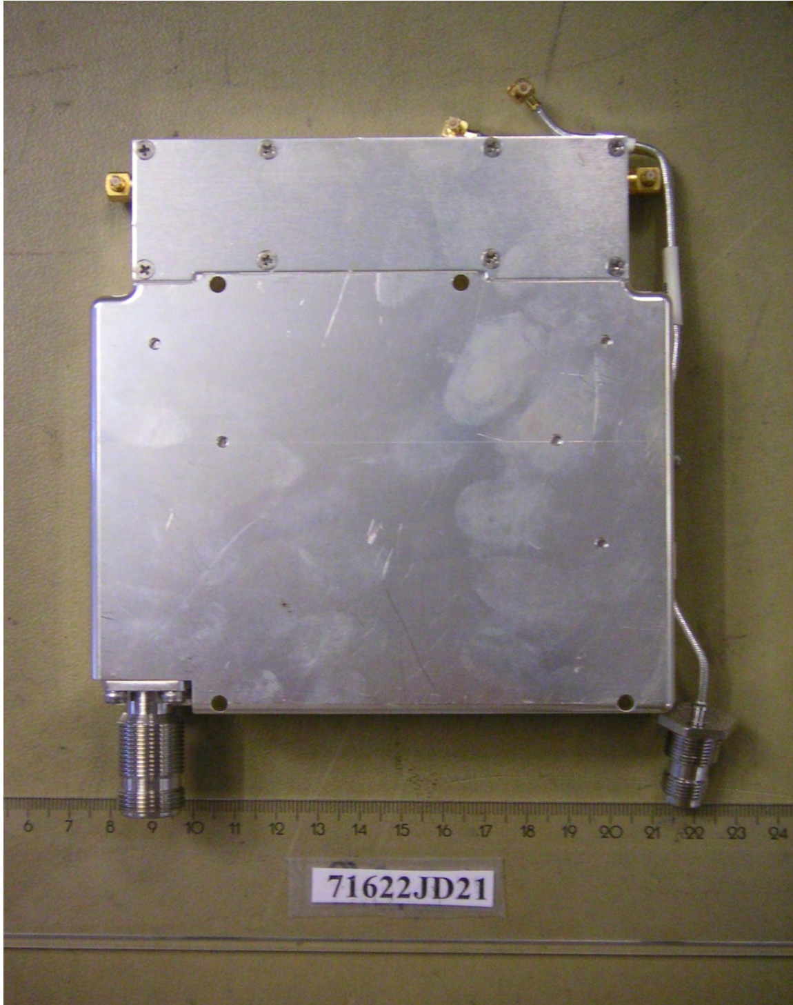
PHT/71622JD21/018 Duplex Filter 1. Back View
