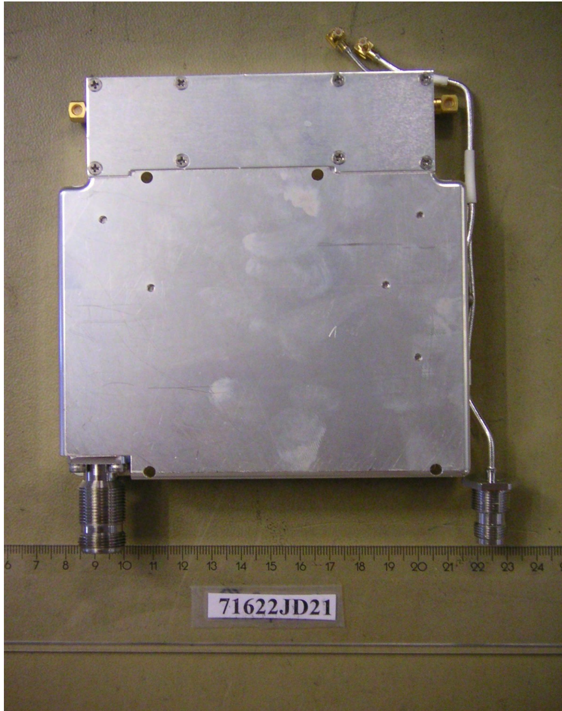
PHT/71622JD21/020 Duplex Filter 2. Back View
