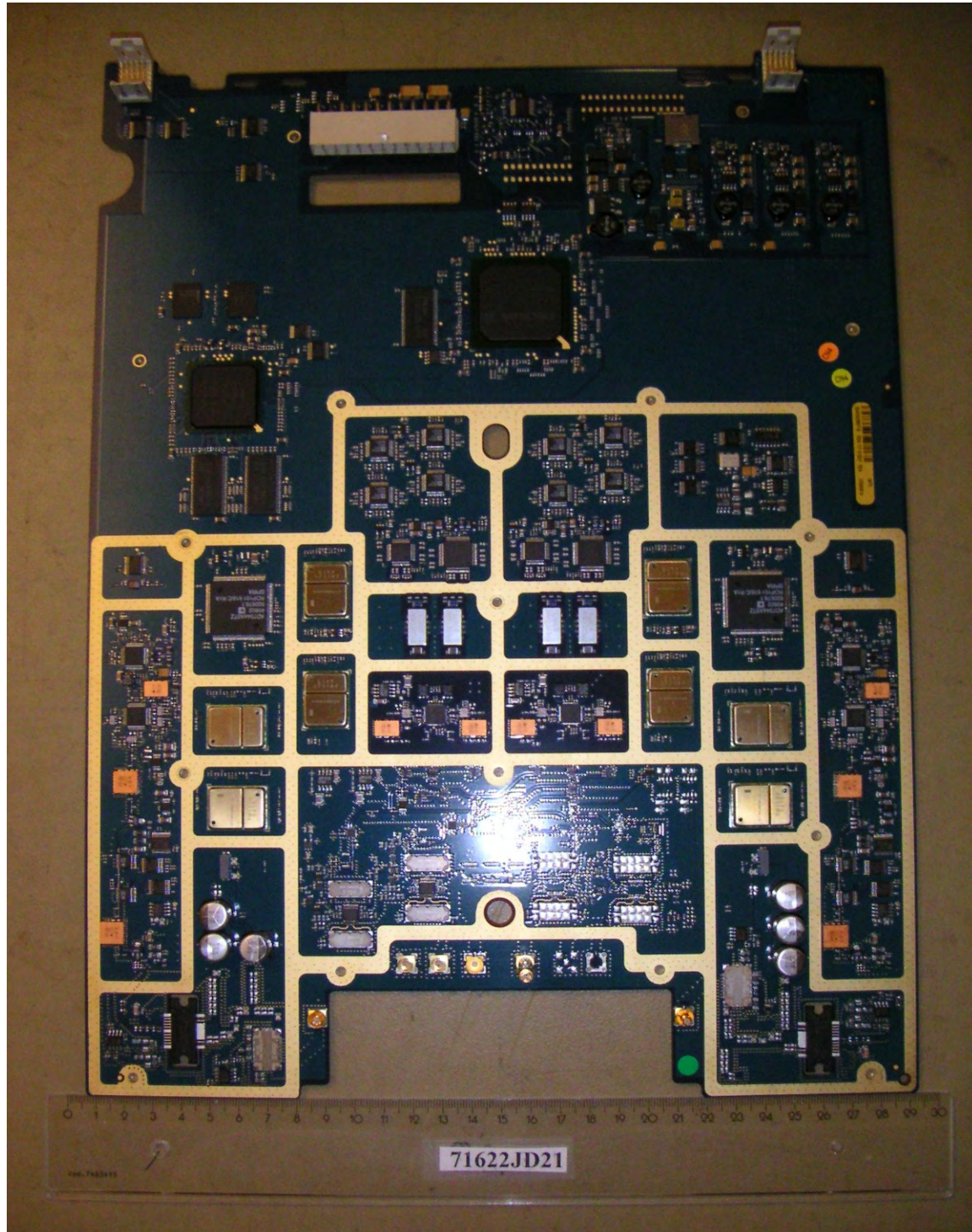
PHT/71622JD21/015 Digital Radio Access Board 2. Front View
