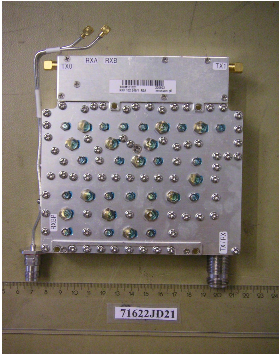
PHT/71622JD21/019 Duplex Filter 2. Front View
