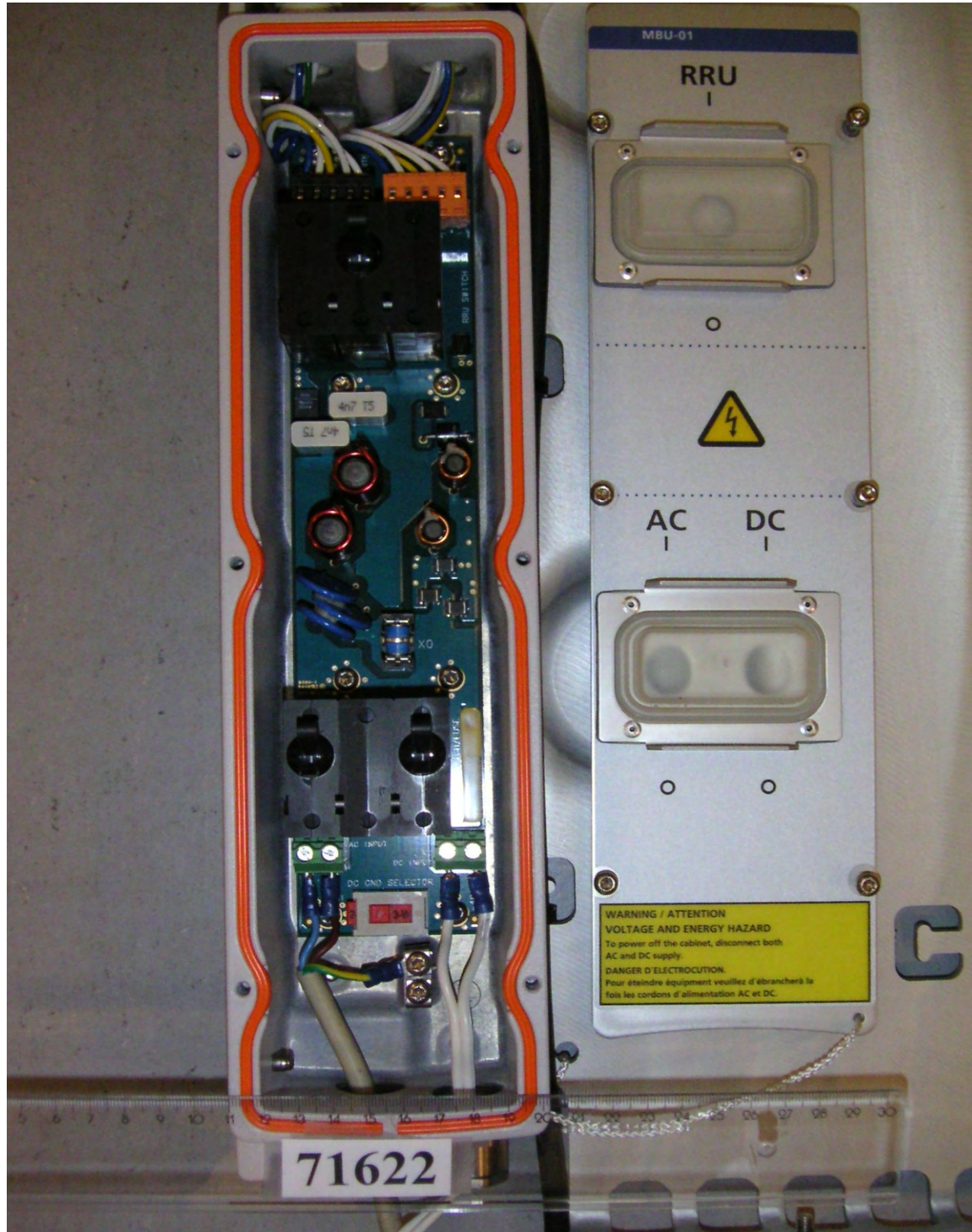
PHT/71622JD21/006 Mounting Base PSU. Internal View
