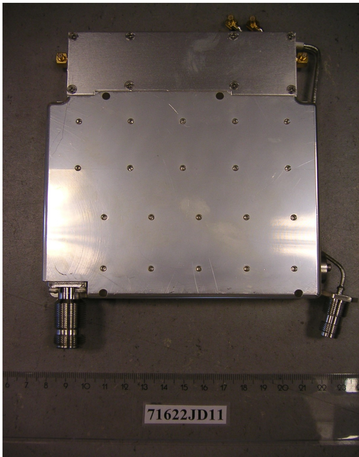
PHT/71622JD11/020 Duplex Filter 2. Back View
