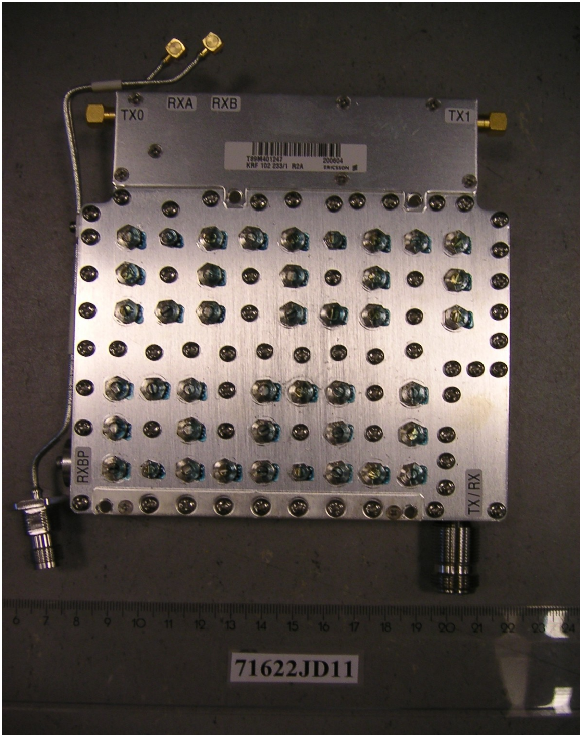
PHT/71622JD11/019 Duplex Filter 2. Front View
