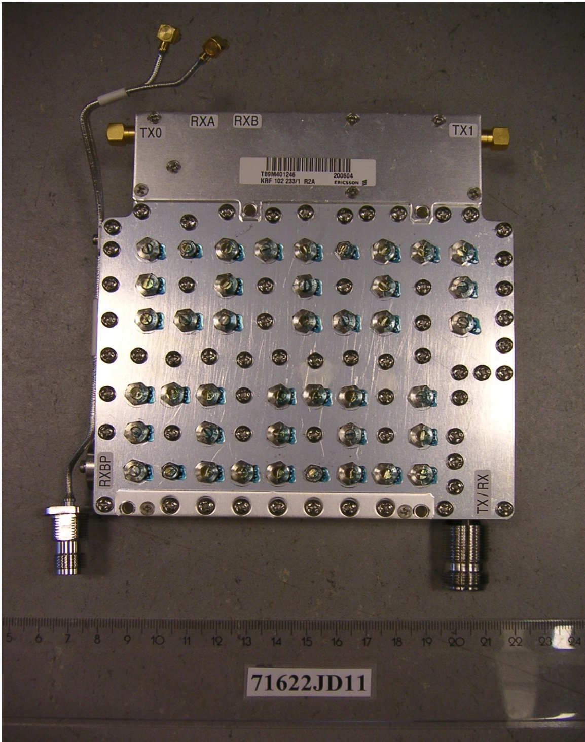
PHT/71622JD11/017 Duplex Filter 1. Front View
