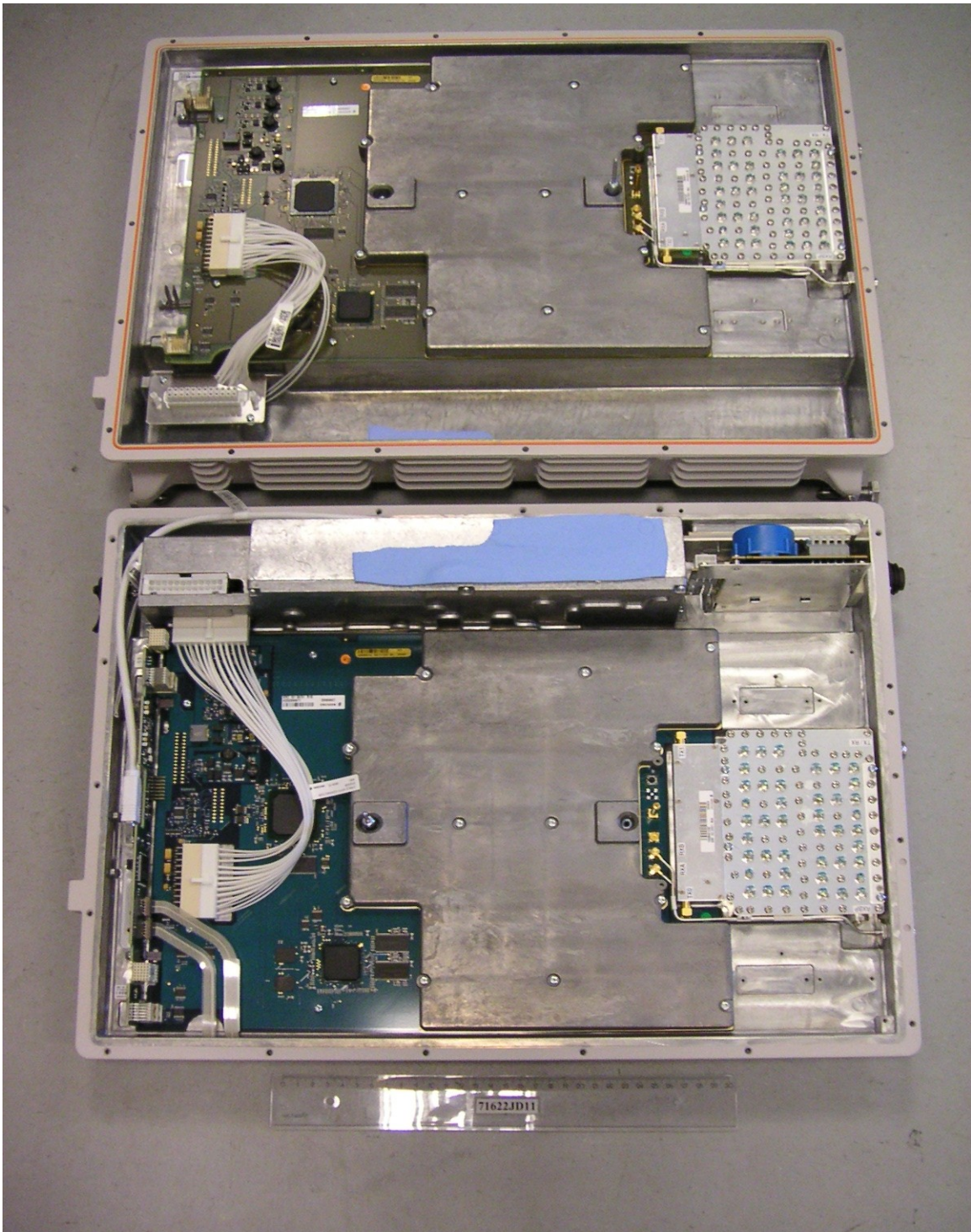
PHT/71622JD11/012 RRU-M19 EDGE. Open View
