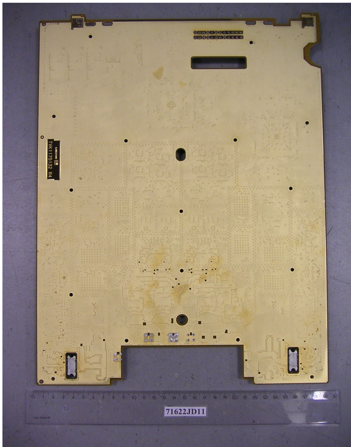
PHT/71622JD11/014 Digital Radio Access Board 1. Back View
