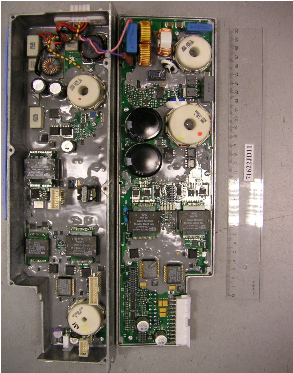
PHT/71622JD11/023 PSU. Internal View
