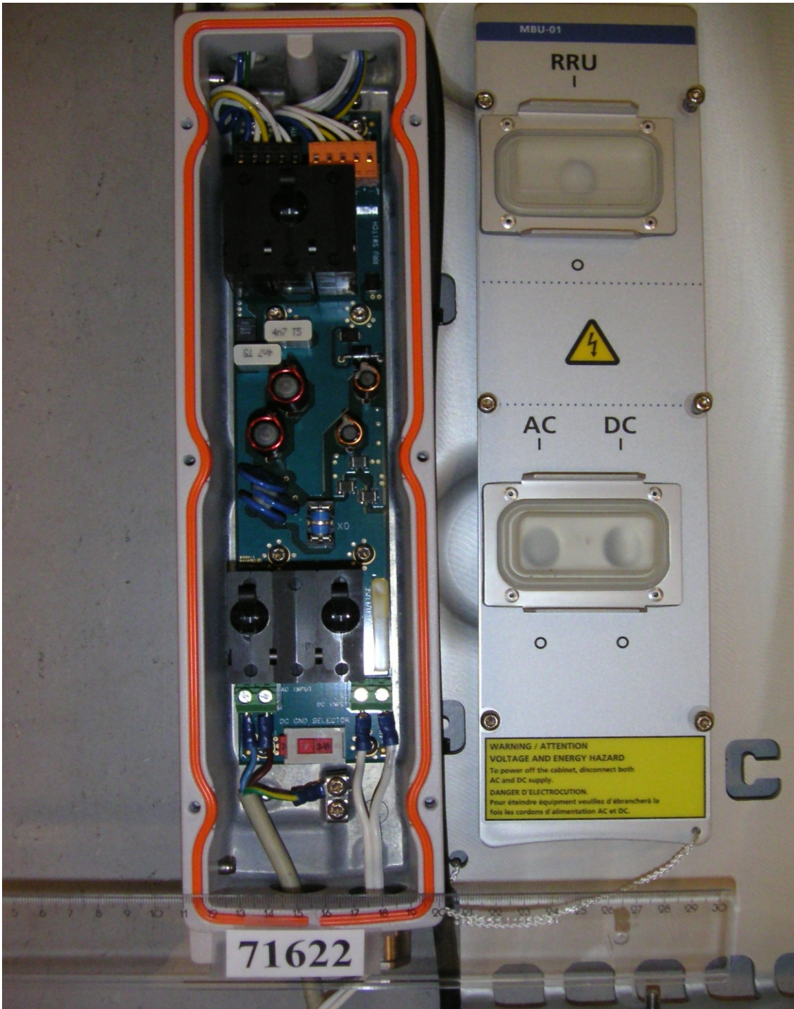
PHT/71622JD11/006 Mounting Base PSU. Internal View
