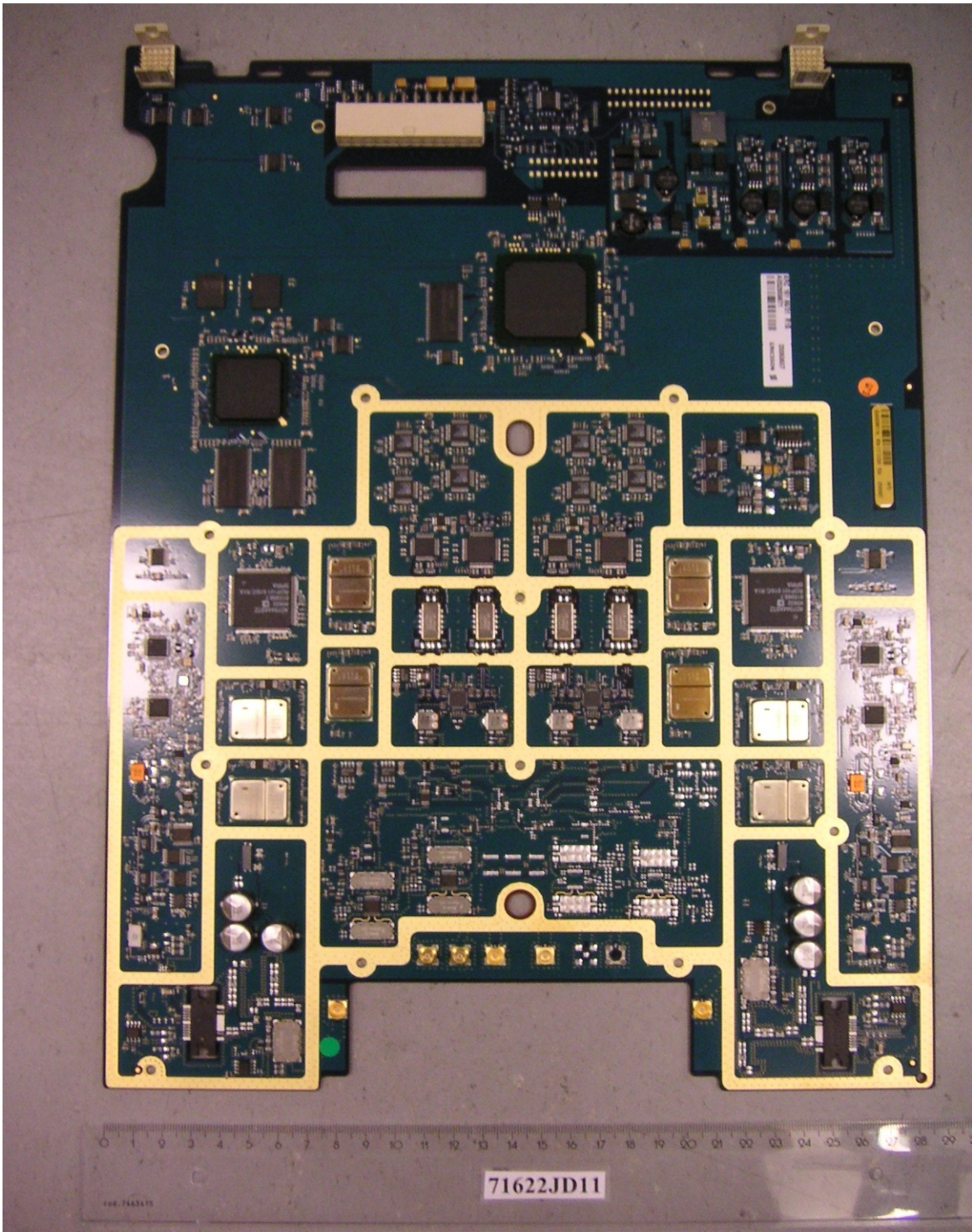
PHT/71622JD11/015 Digital Radio Access Board 2. Front View
