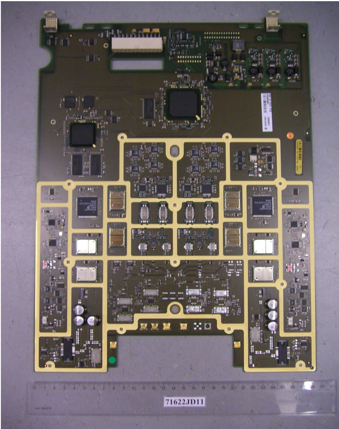
PHT/71622JD11/013 Digital Radio Access Board 1. Front View
