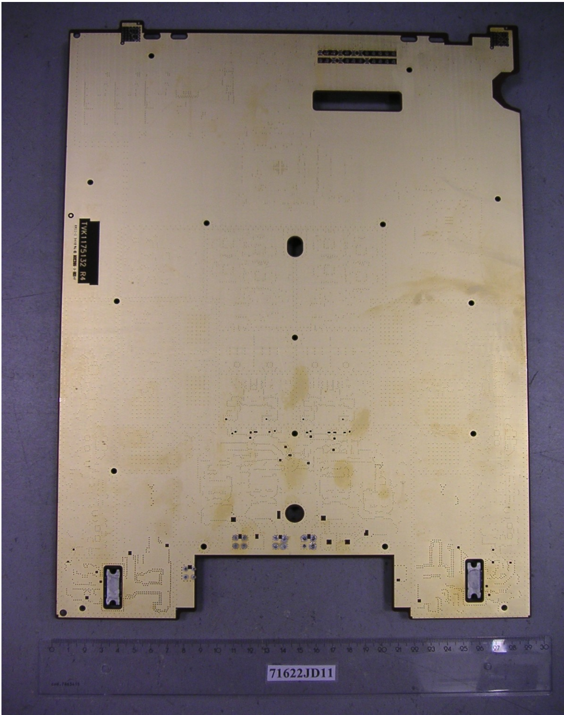
PHT/71622JD11/016 Digital Radio Access Board 2. Back View
