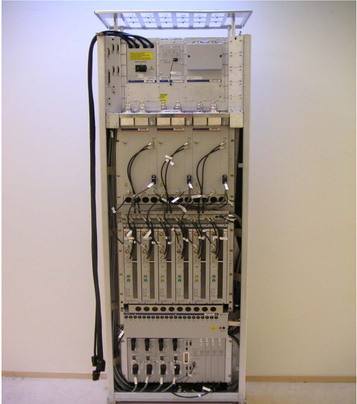
Front View of RBS 2206 GSM 1900 Cabinet
