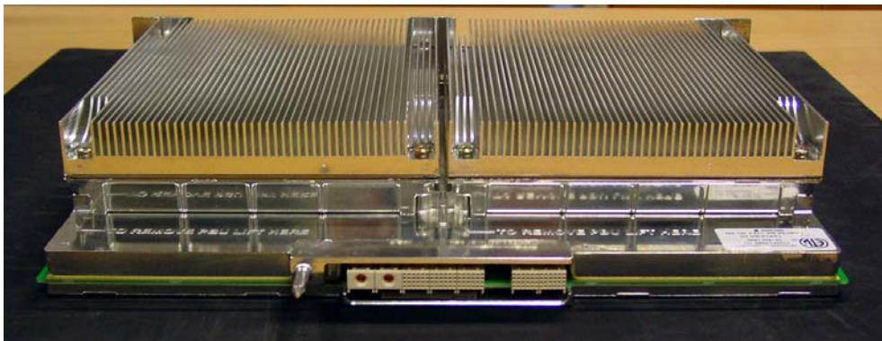
Rear side
