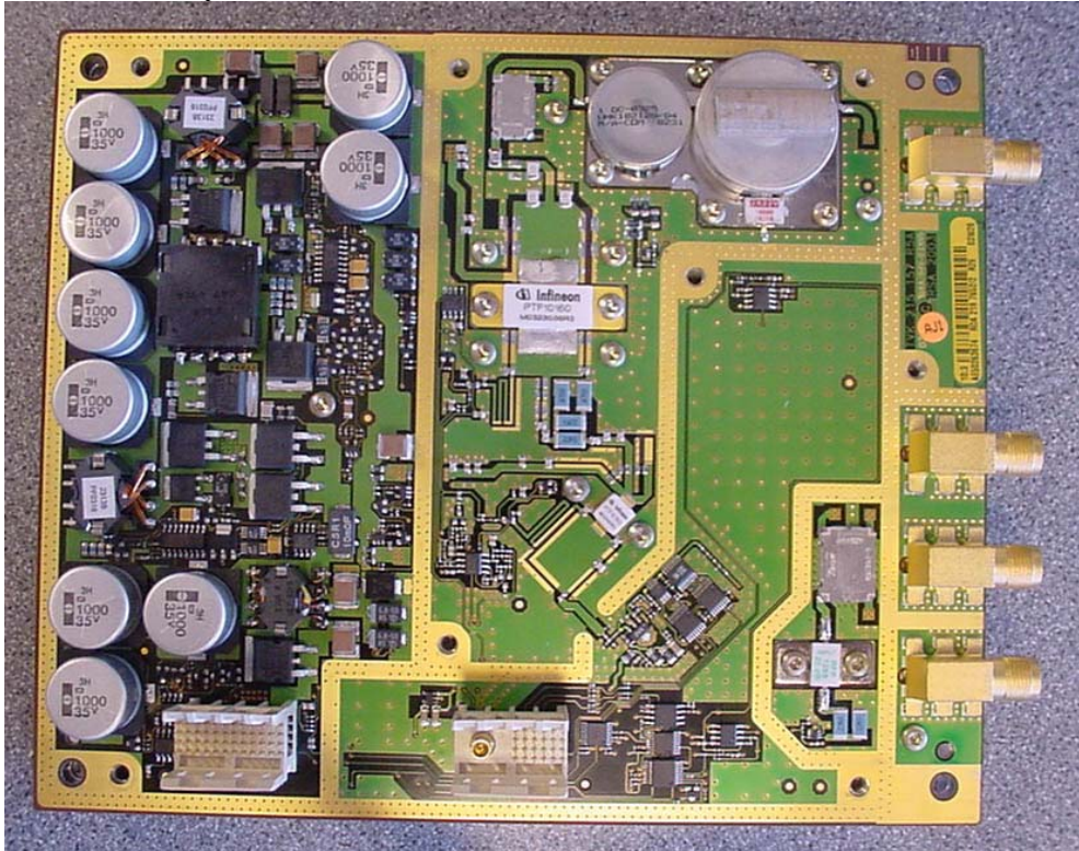
PA1- PCB components side
