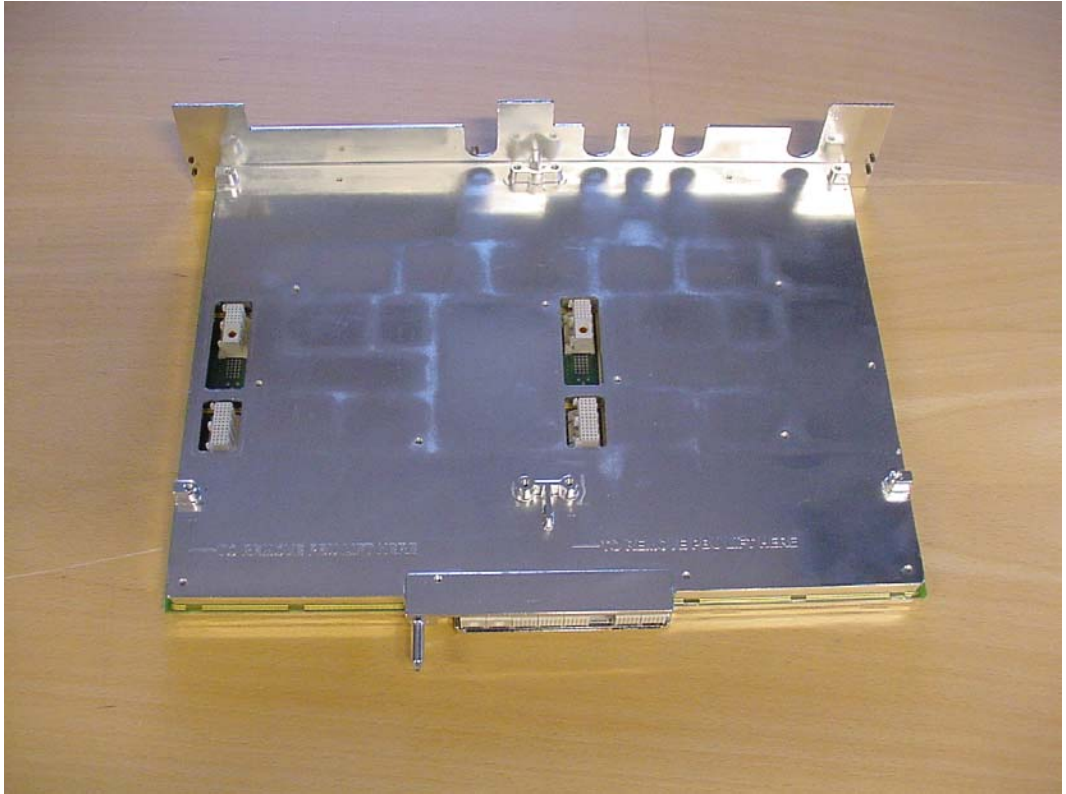
Main board
