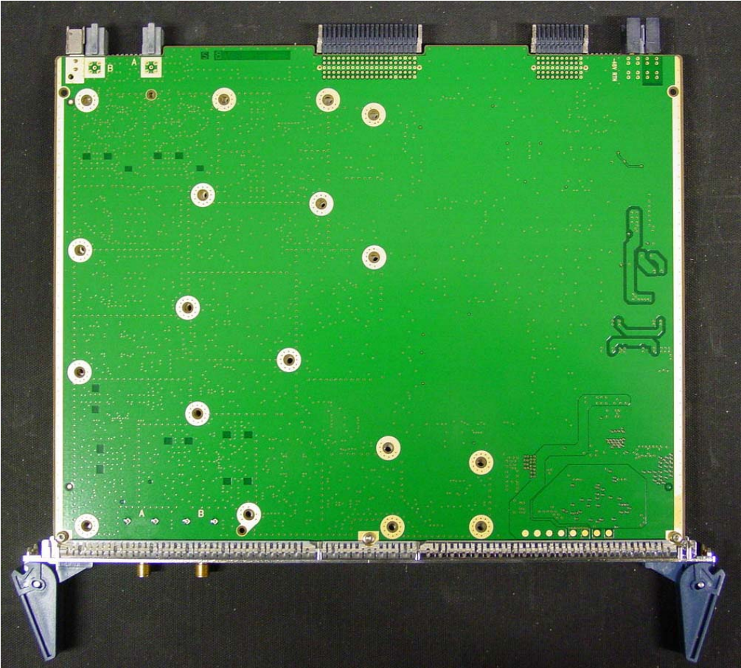
PCB rear side
