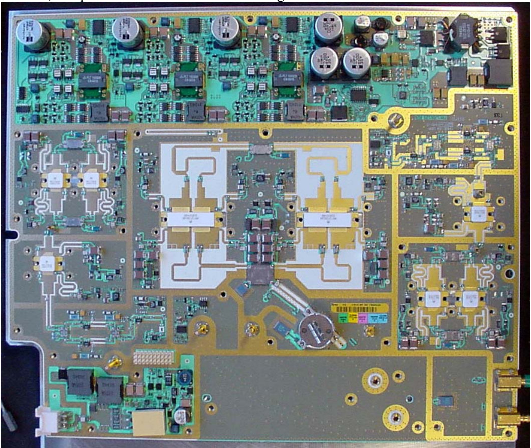
Board 2, component side with transistor holdings and filter removed
