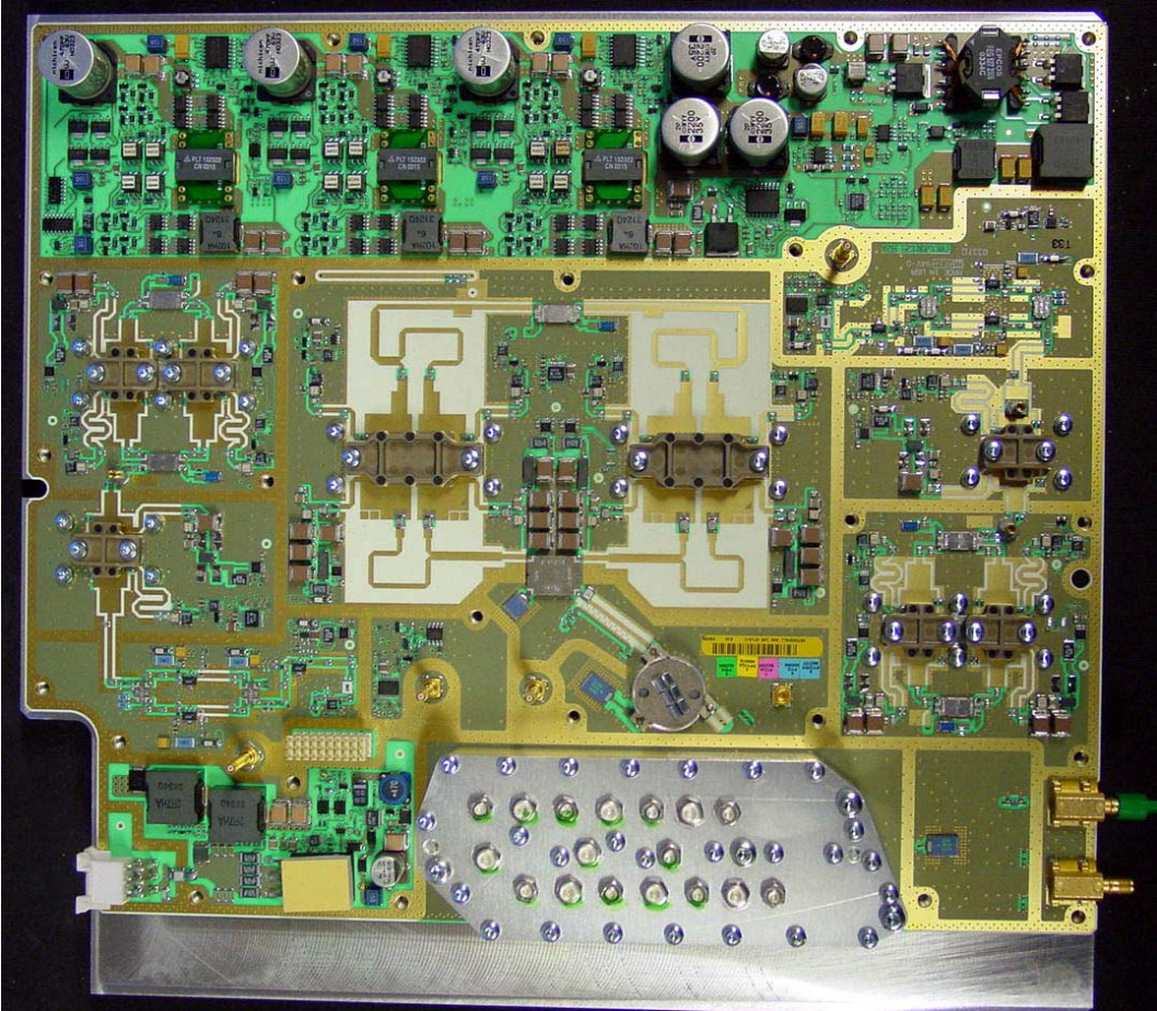
Board 2, component side
