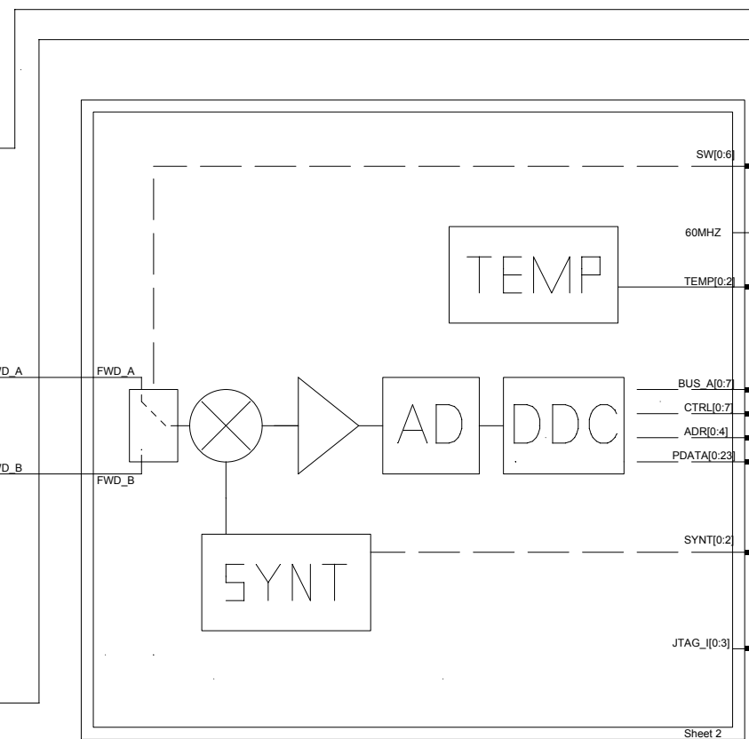
RFPM
