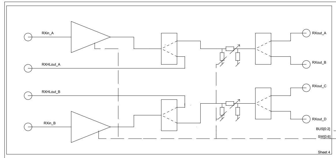
RXPATH
