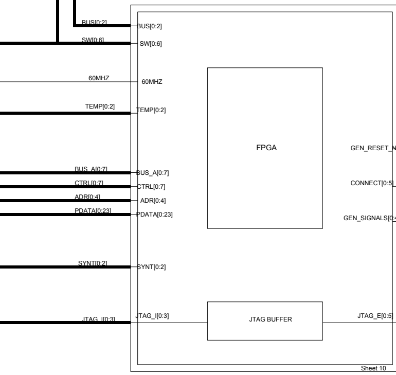
CONTROL
